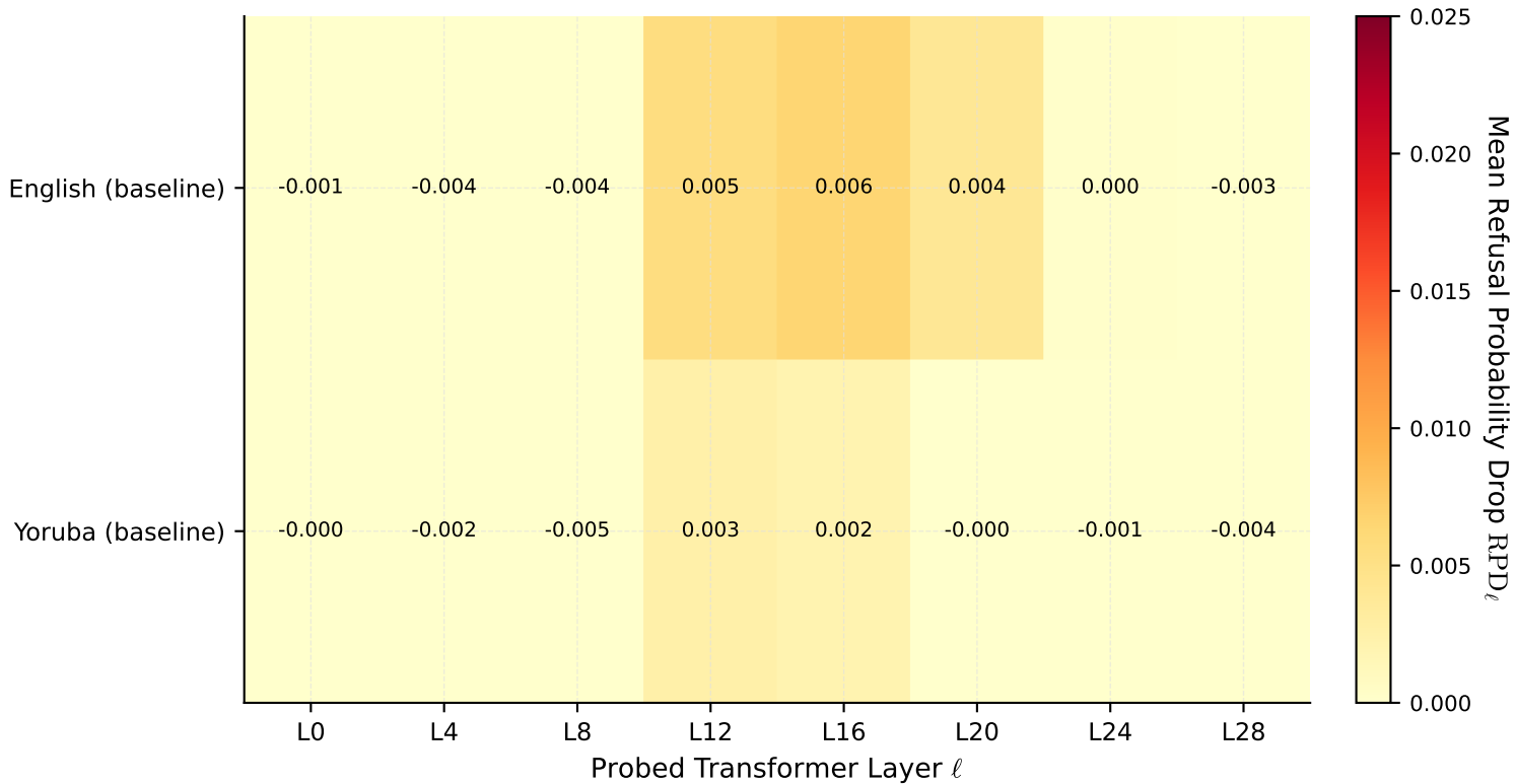
Cross-Lingual Layer Fragility Heatmap ( \text{RPD}_\ell on Unsafe Prompts)
