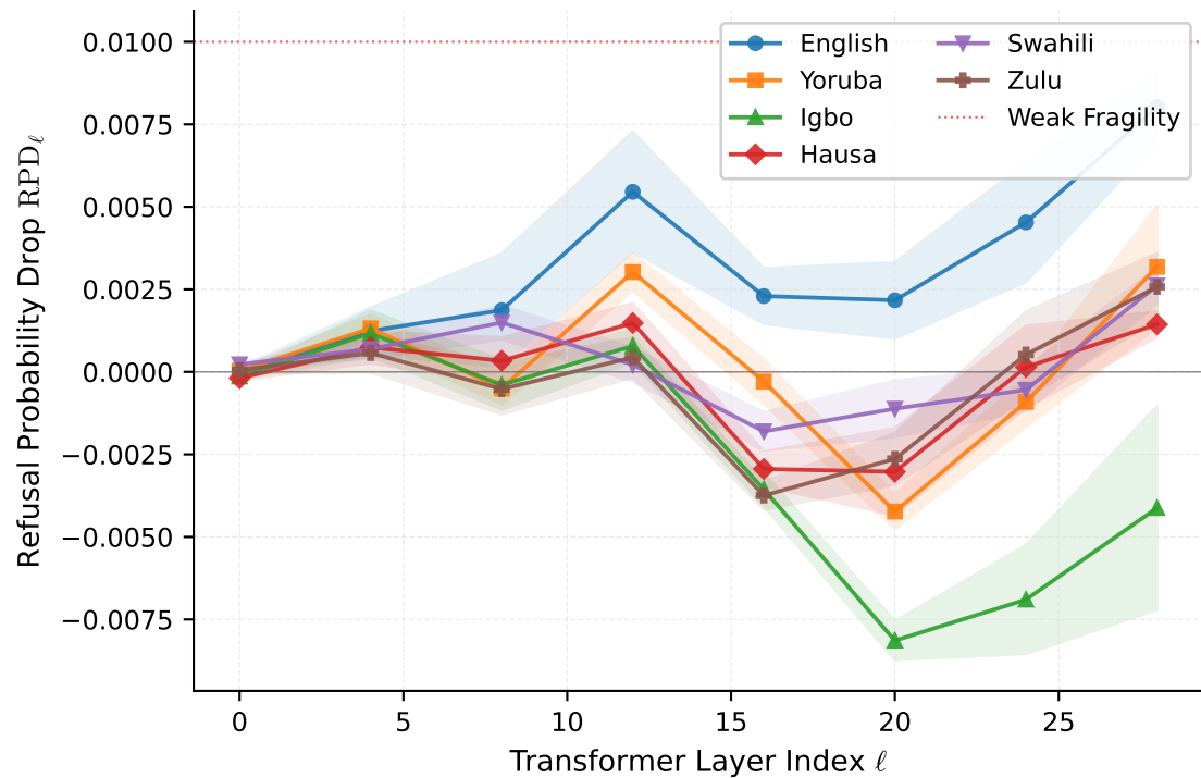
(a) Layer-Wise RPD: Baseline Scaffold
