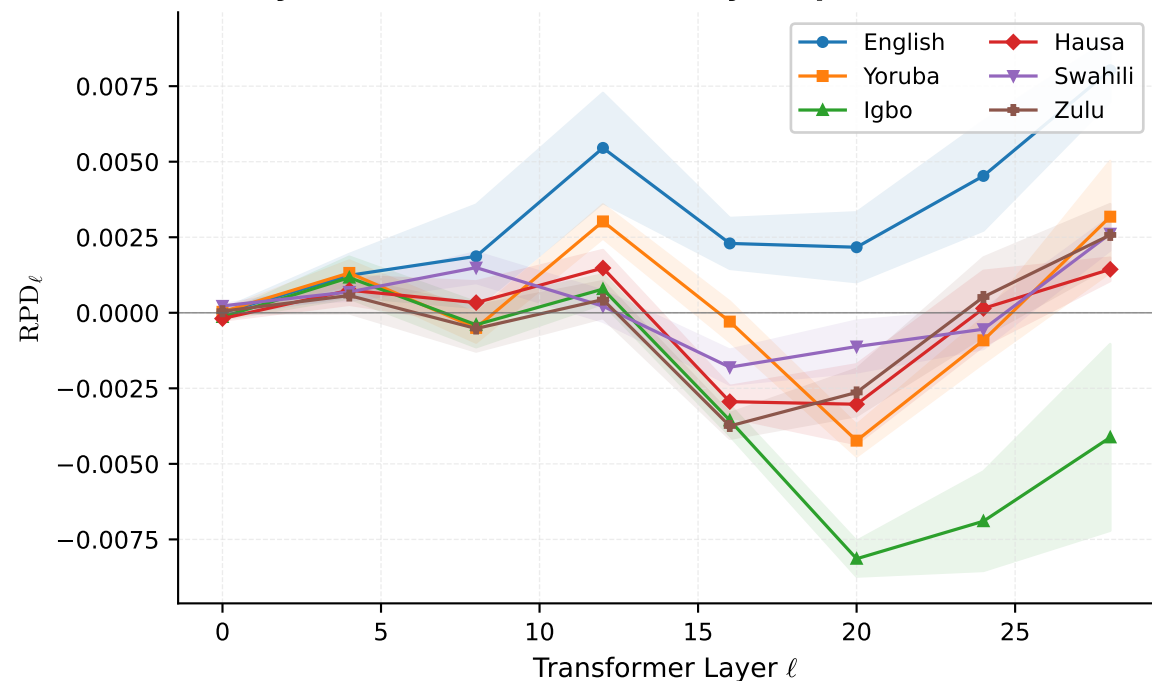
(b) Layer-Wise Refusal Probability Drop \text{RPD}_\ell
