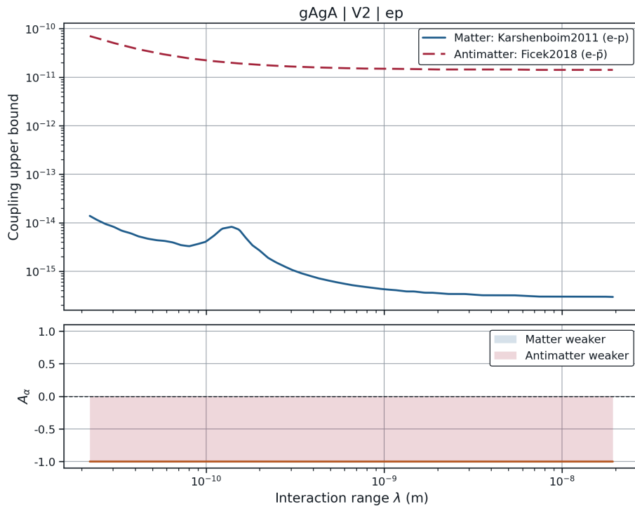
Figure 4.13: Matter-antimatter comparison for the g_{AgA} \cdot V_2 \cdot e\text{-}\bar{p} pair (Karshenboim, 2011, versus Ficek et al. , 2018), the highest asymmetry in the compiled database.
