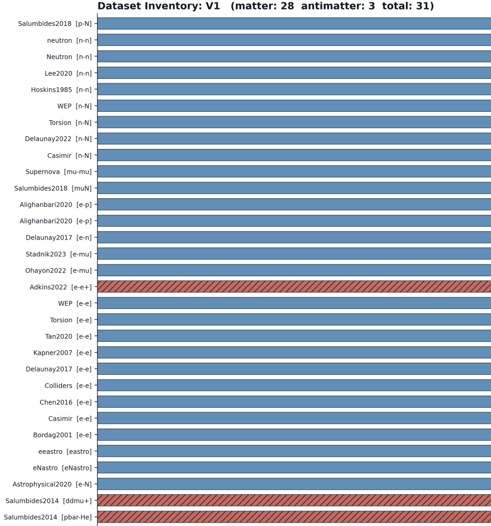
Figure 4.16: Dataset inventory for V_1 .
