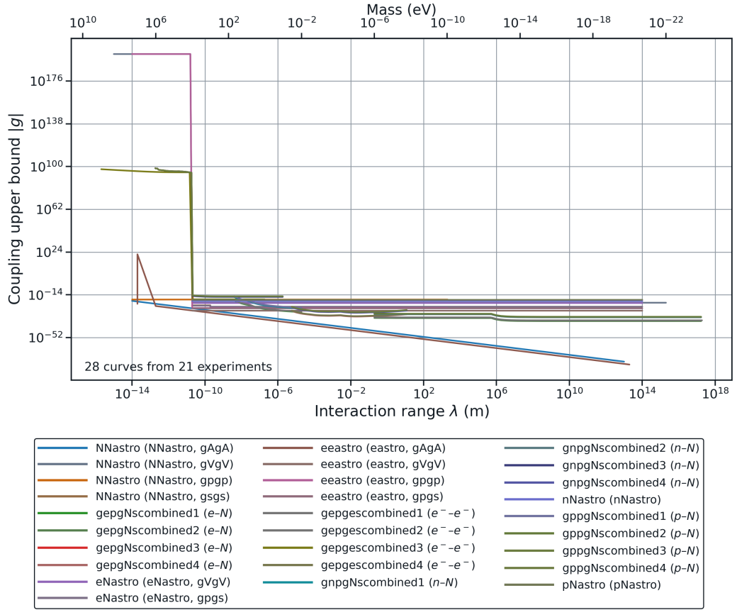
Figure 4.3: Constraint atlas for V_{1a} .
