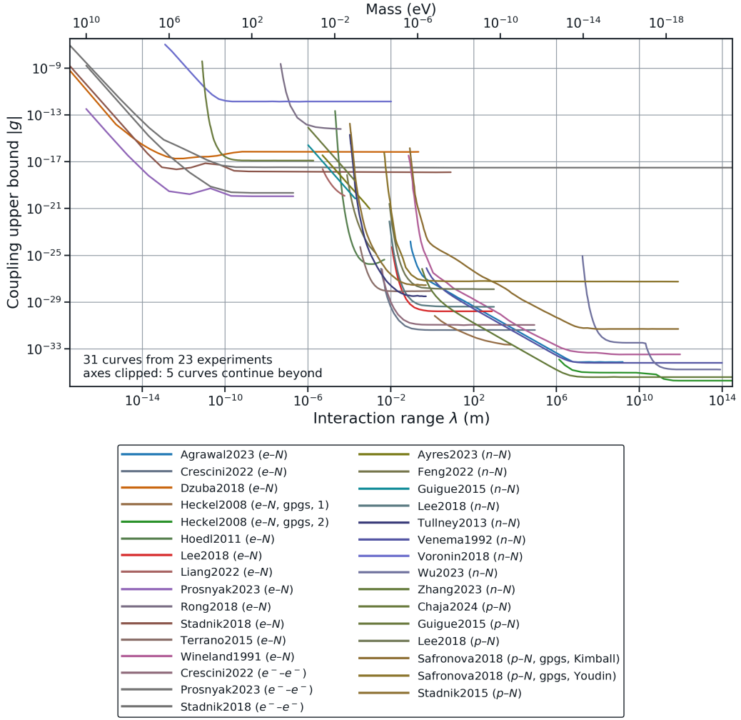
Figure 4.8: Constraint atlas for V_{9+10} .
