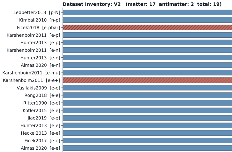
Figure C.2: Dataset inventory for V_2 .
