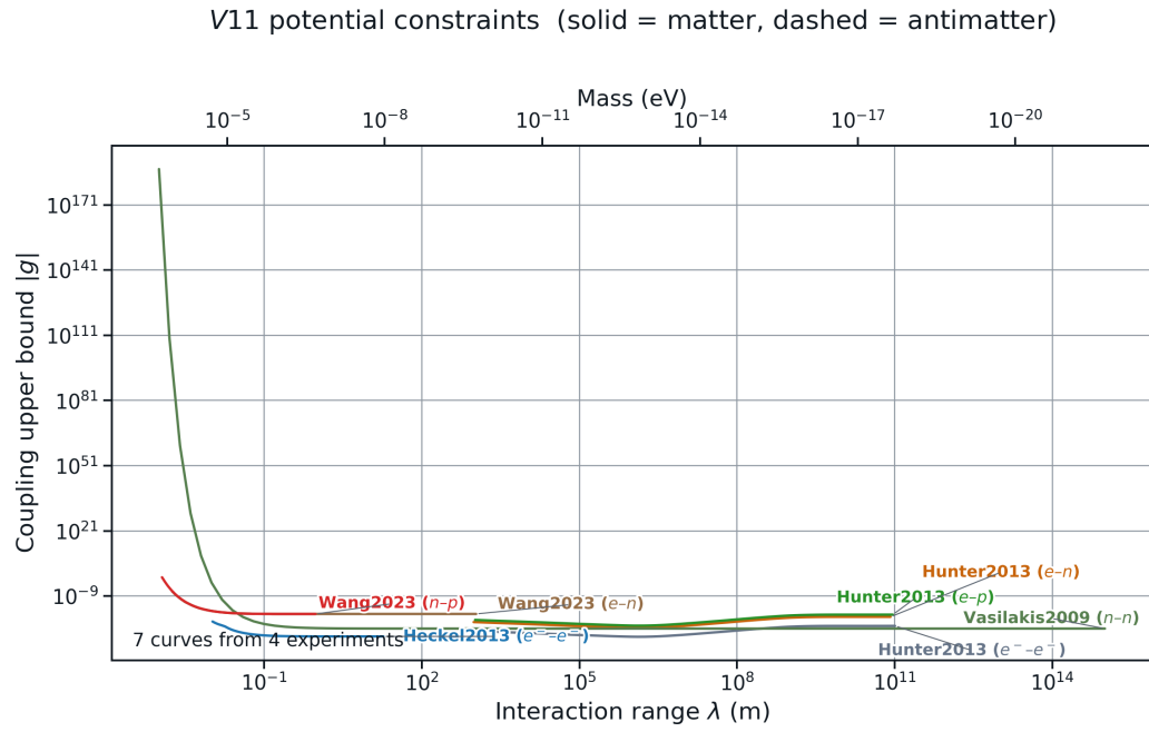
Figure 4.9: Constraint atlas for V_{11} .
