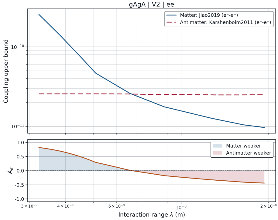
Figure 4.14: Matter–antimatter comparison for the g_{AgA} \cdot V_2 \cdot e-e^+ pair (Jiao et al. , versus Karshenboim, 2011), the lowest asymmetry in the compiled database ( |A_\alpha| = 0.334 ), included alongside Figure 4.13 to show that the analysis does not produce a saturated asymmetry for every pair by construction.
