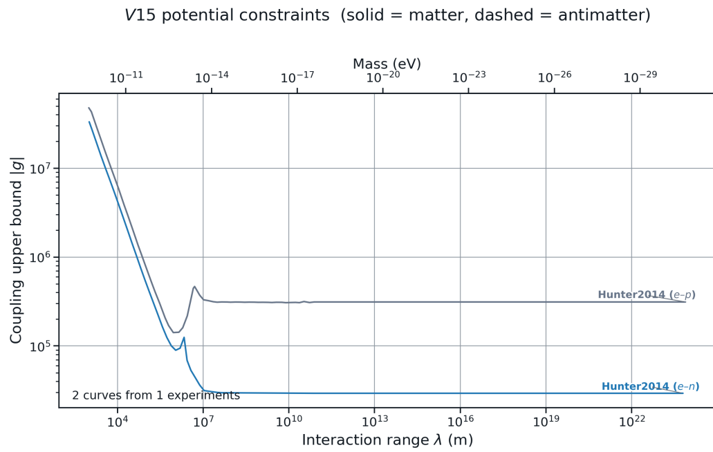
Figure 4.11: Constraint atlas for V_{15} .
