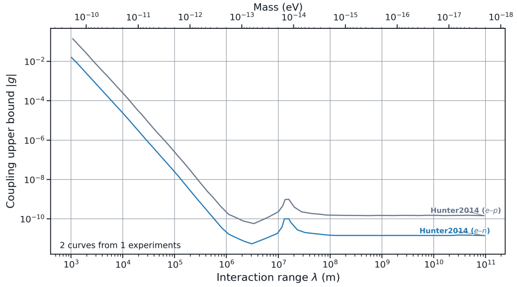
Figure 4.12: Constraint atlas for V_{16} .
