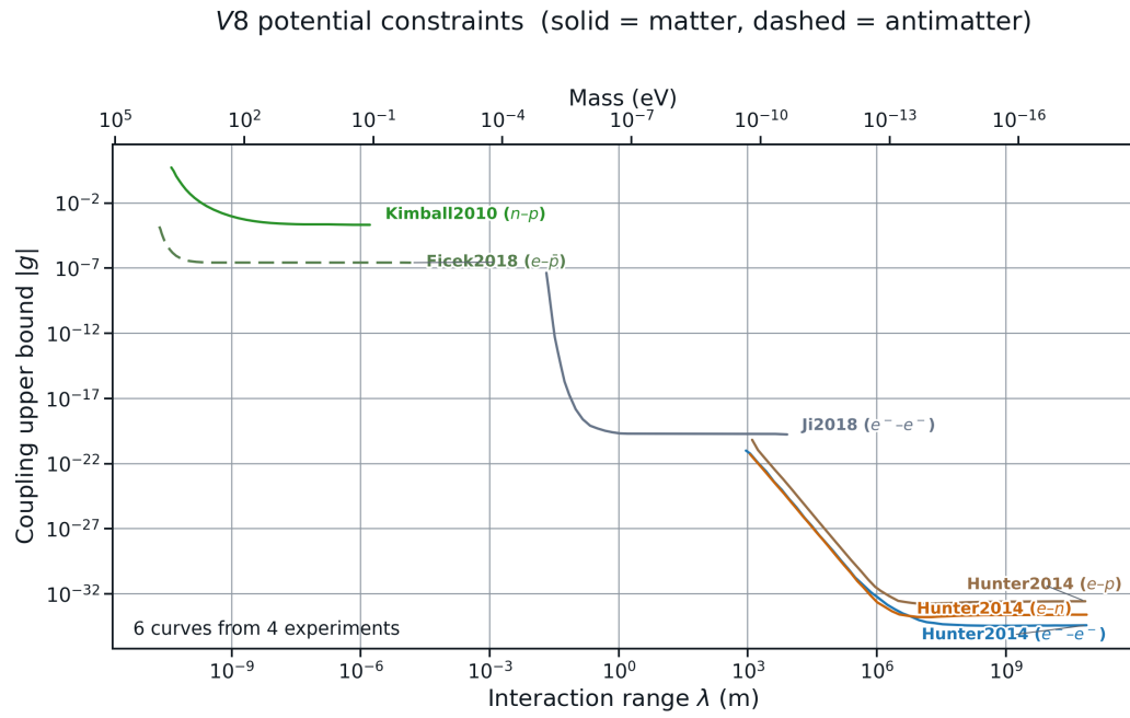
Figure 4.7: Constraint atlas for V_8 .
