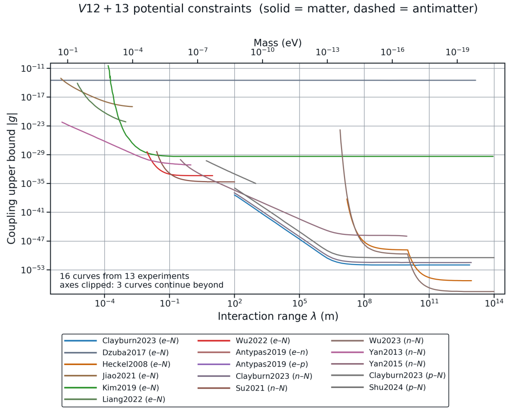
Figure 4.10: Constraint atlas for V_{12+13} .
