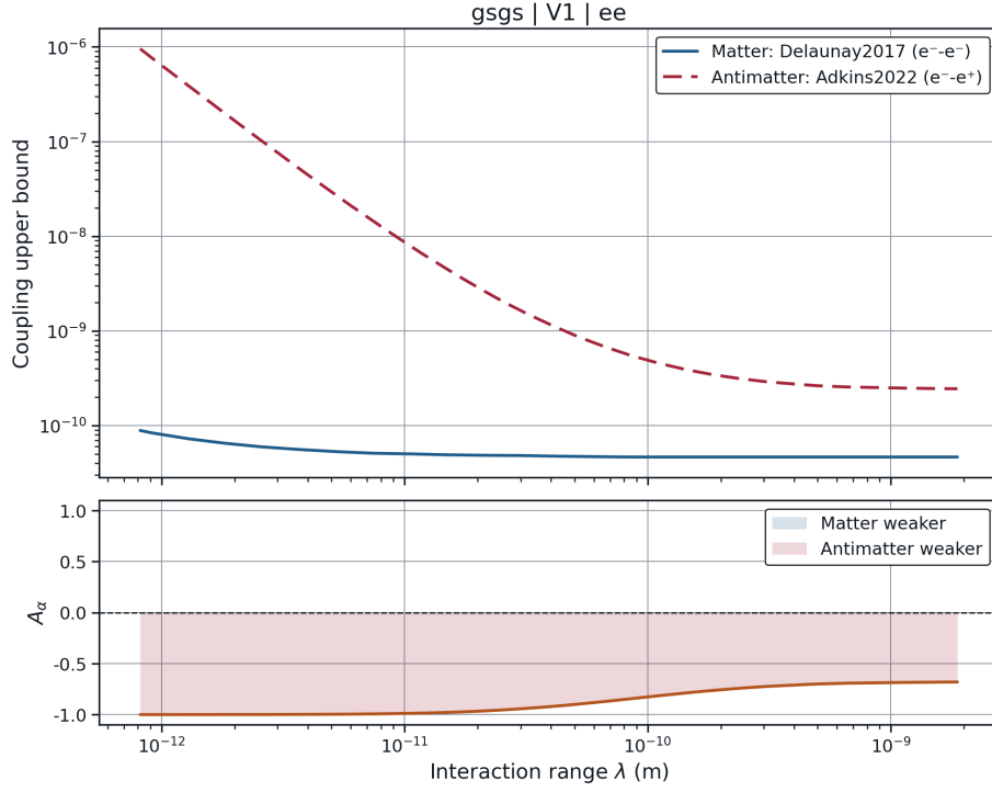
Figure 4.15: Matter–antimatter comparison for the g_s g_s \cdot V_1 \cdot e-e^+ pair (Delaunay et al. , 2017, versus Adkins et al. , 2022), the only currently matched V_1 pair and, per the discussion following Table 4.3, a CPT-even channel whose high asymmetry is attributable entirely to the sensitivity gap between the two measurements rather than to any CPT-violating physics.
