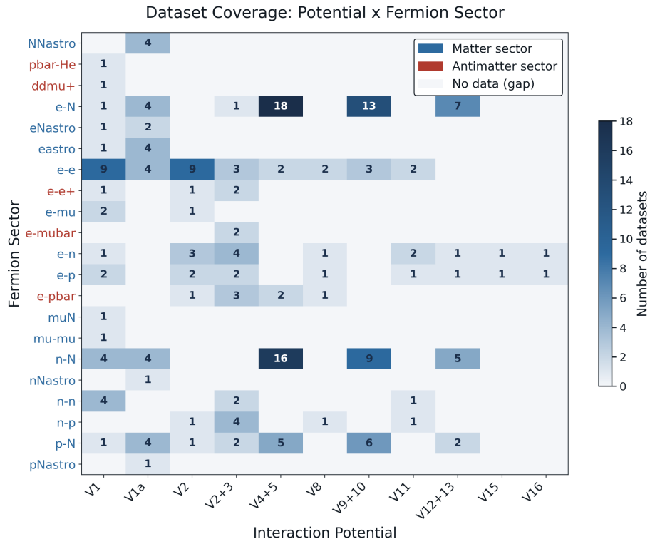
Figure 4.19: Dataset count by potential and sector; antimatter-sector rows are highlighted, visually reproducing the gaps quantified in Tables 4.4 and 4.5.
