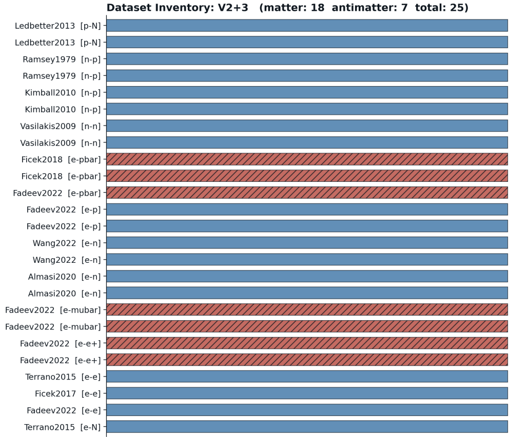
Figure C.3: Dataset inventory for V_{2+3} .
