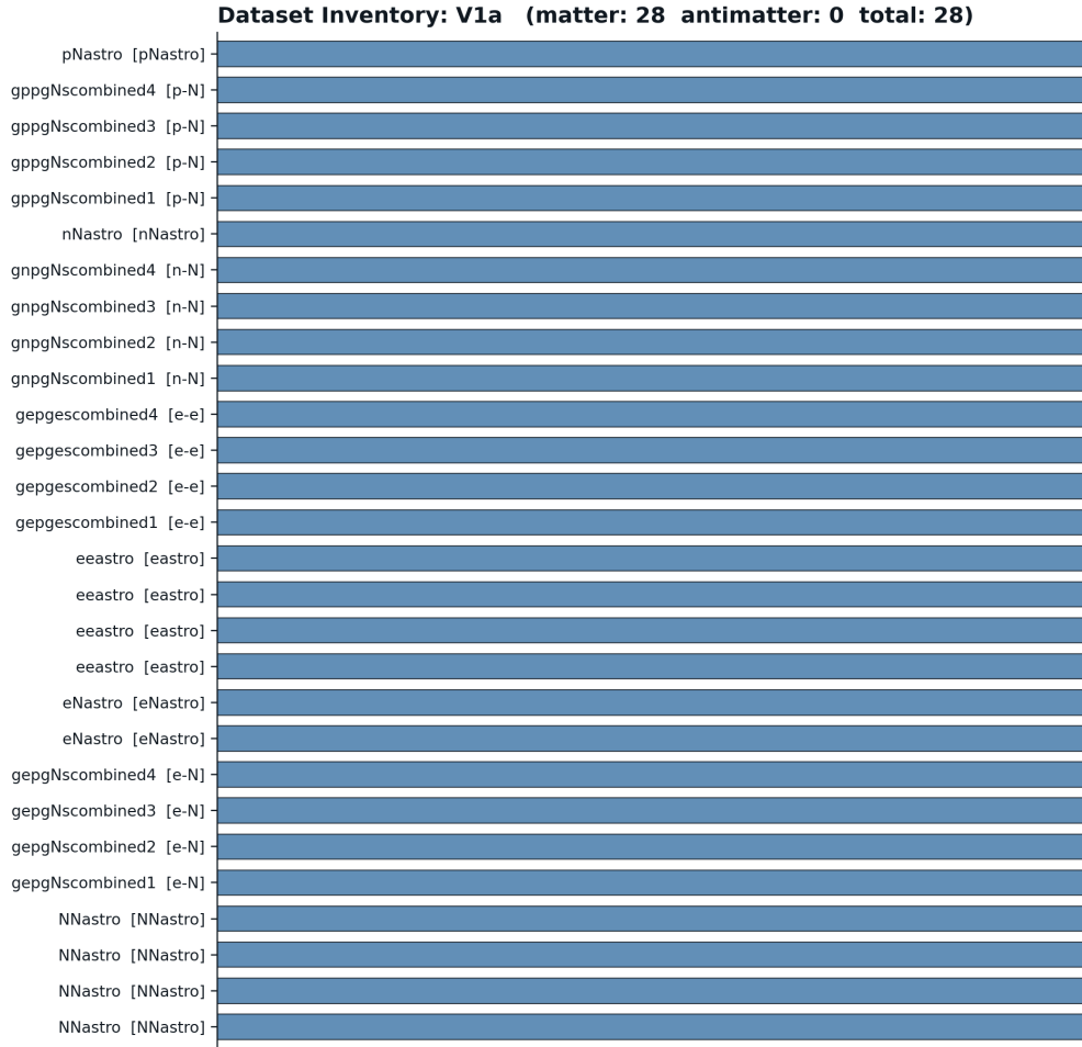
Figure C.1: Dataset inventory for V_{1a} .
