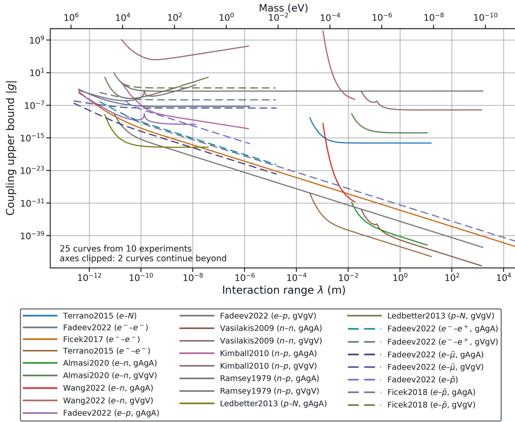
Figure 4.5: Constraint atlas for V_{2+3} .
