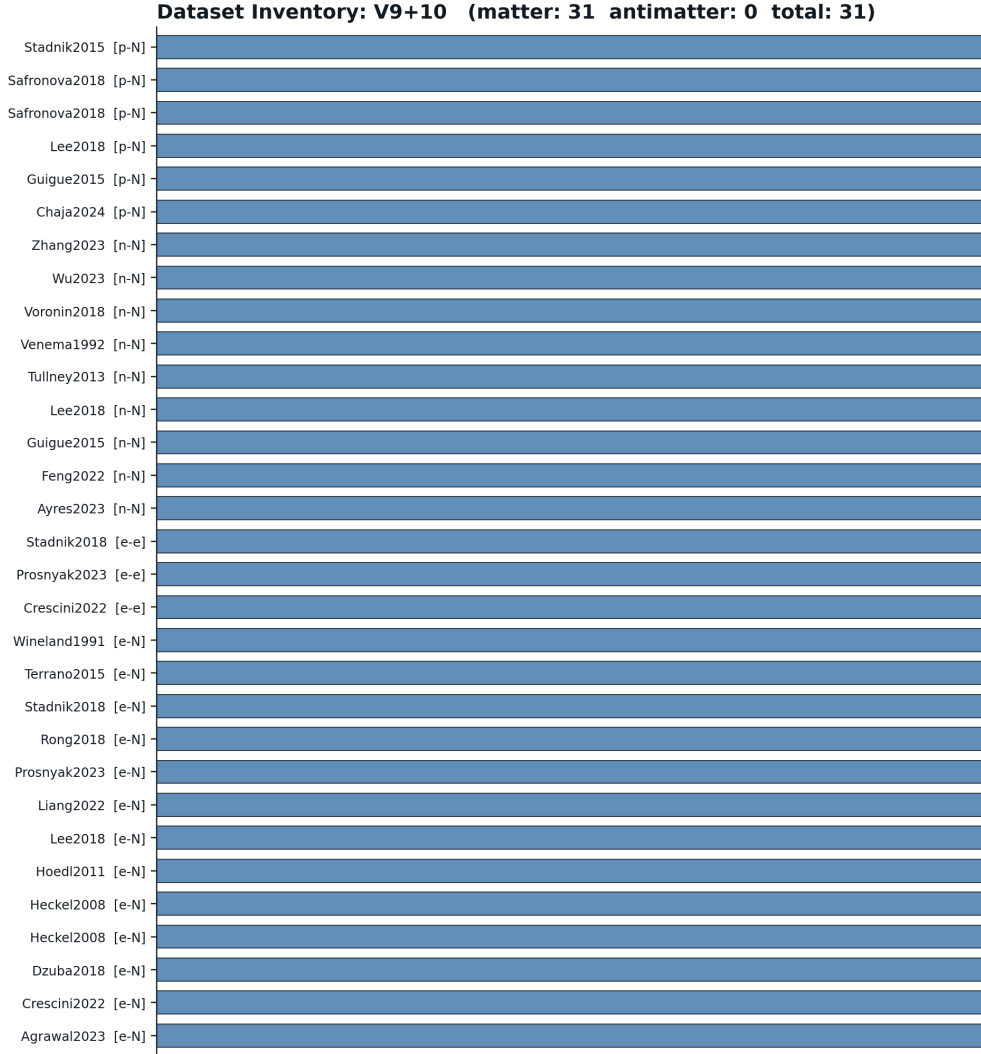
Figure 4.18: Dataset inventory for V_{9+10} .
