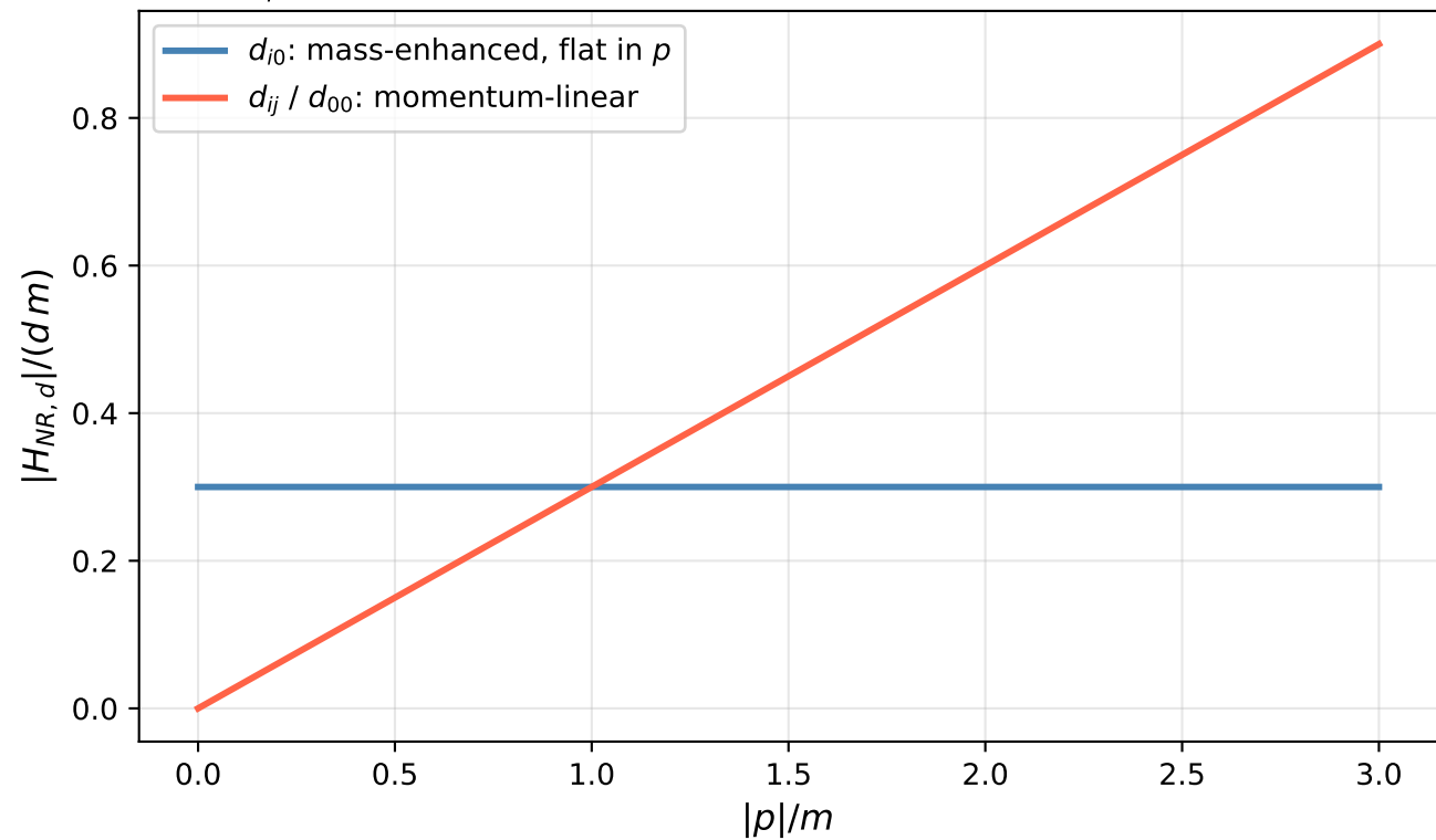
d_{\mu\nu} contributions: mass-enhanced vs. momentum-dependent
