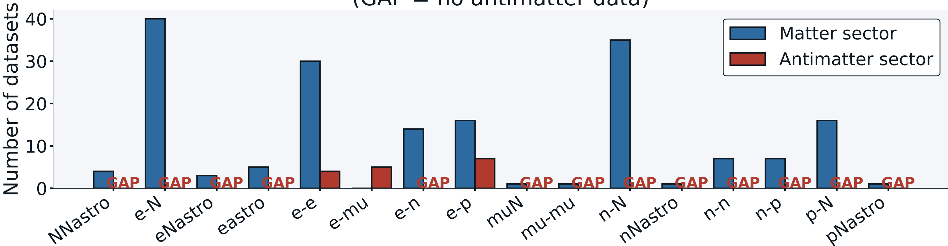
Matter vs Antimatter Dataset Coverage per Fermion Sector (GAP = no antimatter data)
