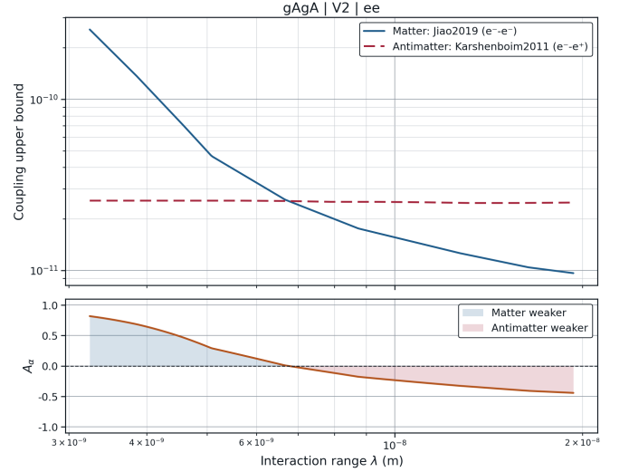
FIG. 3. Matter–antimatter comparison for the g_{AgA} \cdot V_2 \cdot e\text{-}e^+ pair, the lowest asymmetry in the database ( |A_\alpha| = 0.3336 ). The two sectors are probed at comparable sensitivity here, making this the most informative pair in the present database despite its smaller asymmetry.
