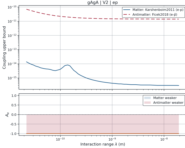
FIG. 2. Matter–antimatter comparison for the g_{AgA} \cdot V_2 \cdot e\text{-}\bar{p} pair, the highest asymmetry in the database ( |A_\alpha| = 0.9998 ). The two bounds differ by orders of magnitude in sensitivity over the overlapping range, which is sufficient on its own to saturate A_\alpha .
