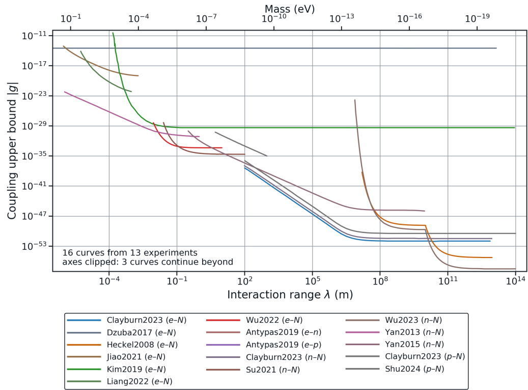
Figure 4.11: Constraint atlas for V_{12+13} .
