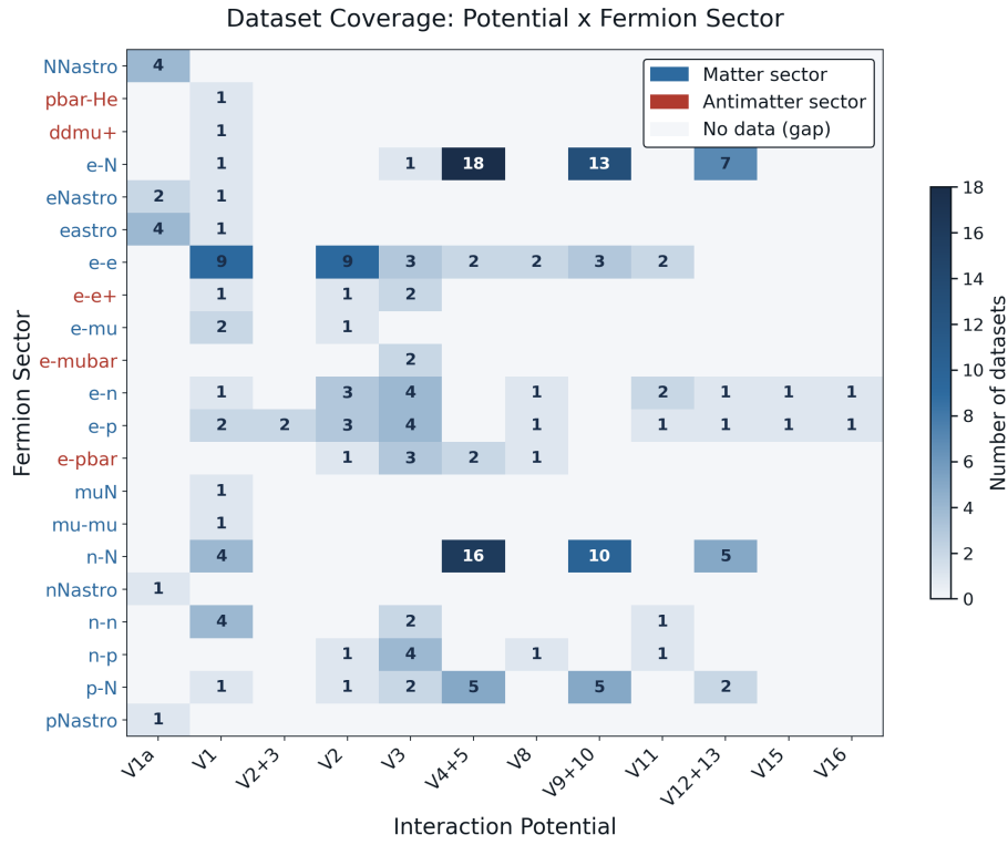
Figure 4.20: Dataset count by potential and sector; antimatter-sector rows are highlighted. Cells count independent bounds, not dataset files, so totals fall below those in Tables 4.4 and 4.5; the gaps identified are the same.
