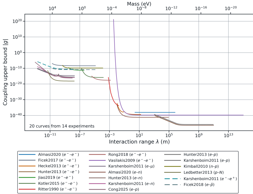
Figure 4.4: Constraint atlas for V_2 .
