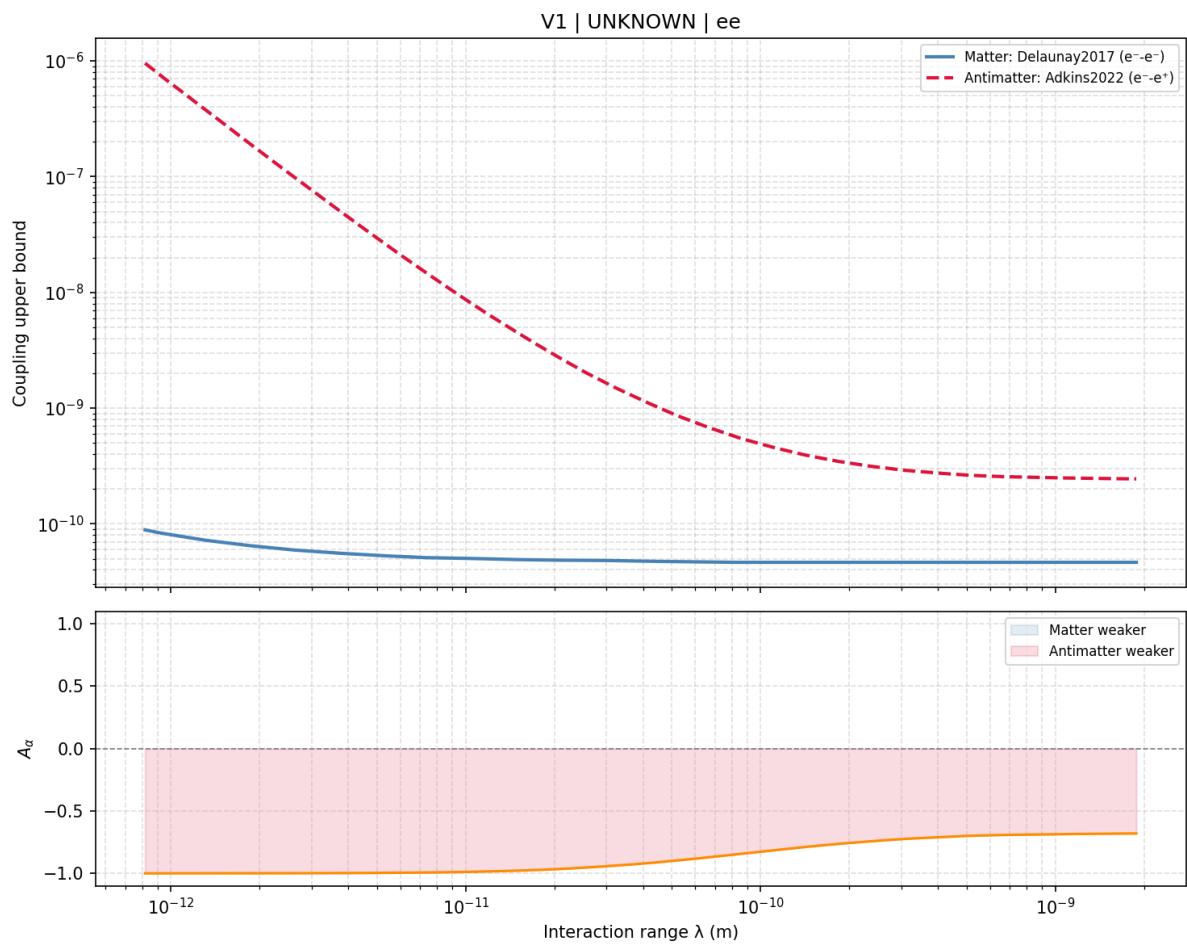
Figure: Coupling upper bounds vs interaction range \lambda (top panel) and asymmetry parameter A_\alpha (bottom panel) for the ee sector under UNKNOWN potential.
