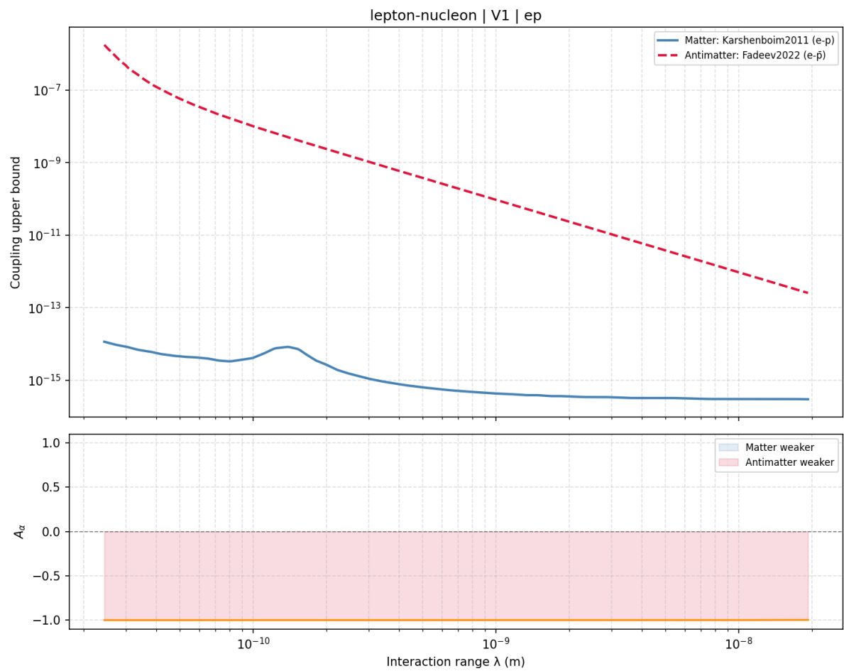
Figure: Coupling upper bounds vs interaction range \lambda (top panel) and asymmetry parameter A_\alpha (bottom panel) for the ep sector under V1 potential.
