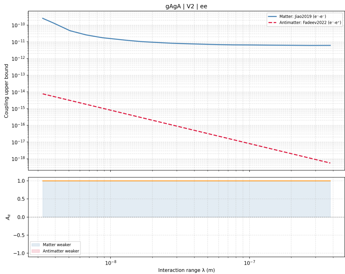
Figure: Coupling upper bounds vs interaction range \lambda (top panel) and asymmetry parameter A_\alpha (bottom panel) for the ee sector under V2 potential.
