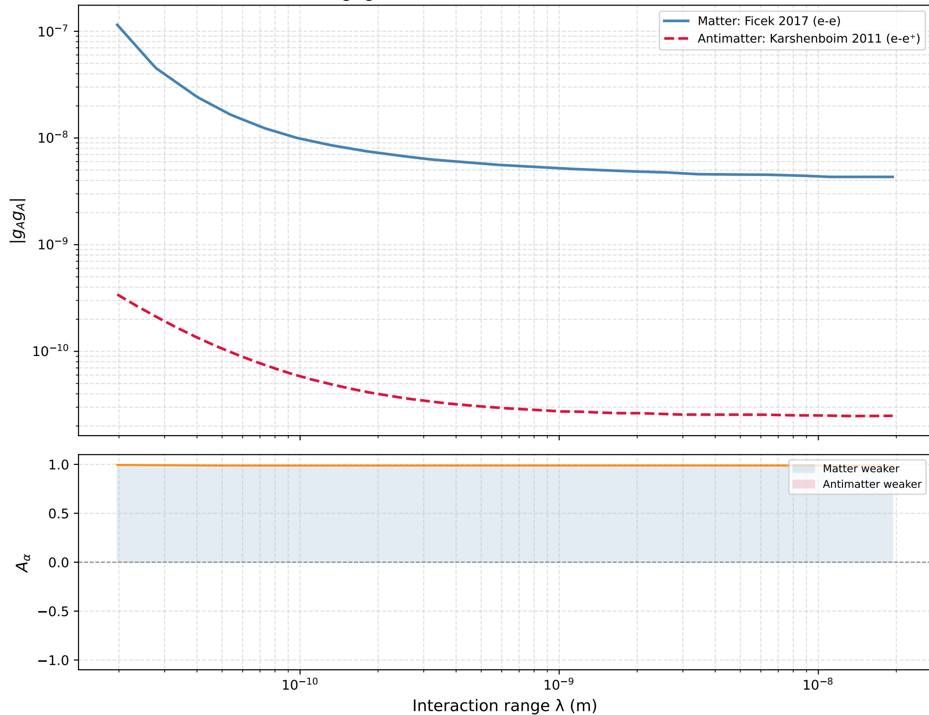
V2 gAgA — matter vs antimatter constraints
