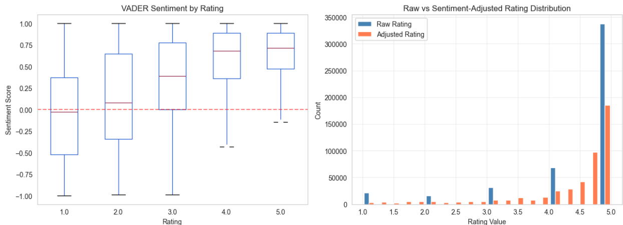
Figure 4. sentiment_analysis.png
