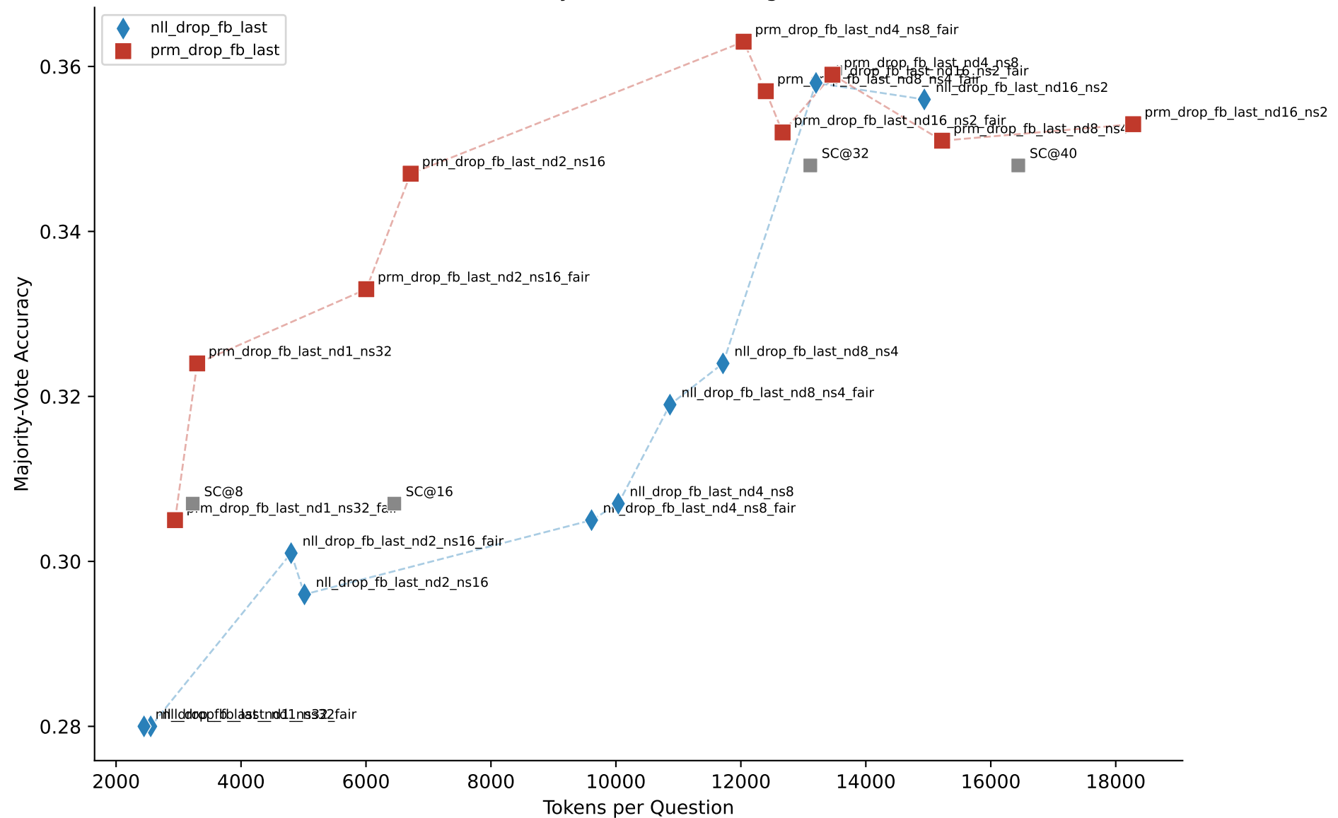
Efficiency Frontier: Multi-Signal
