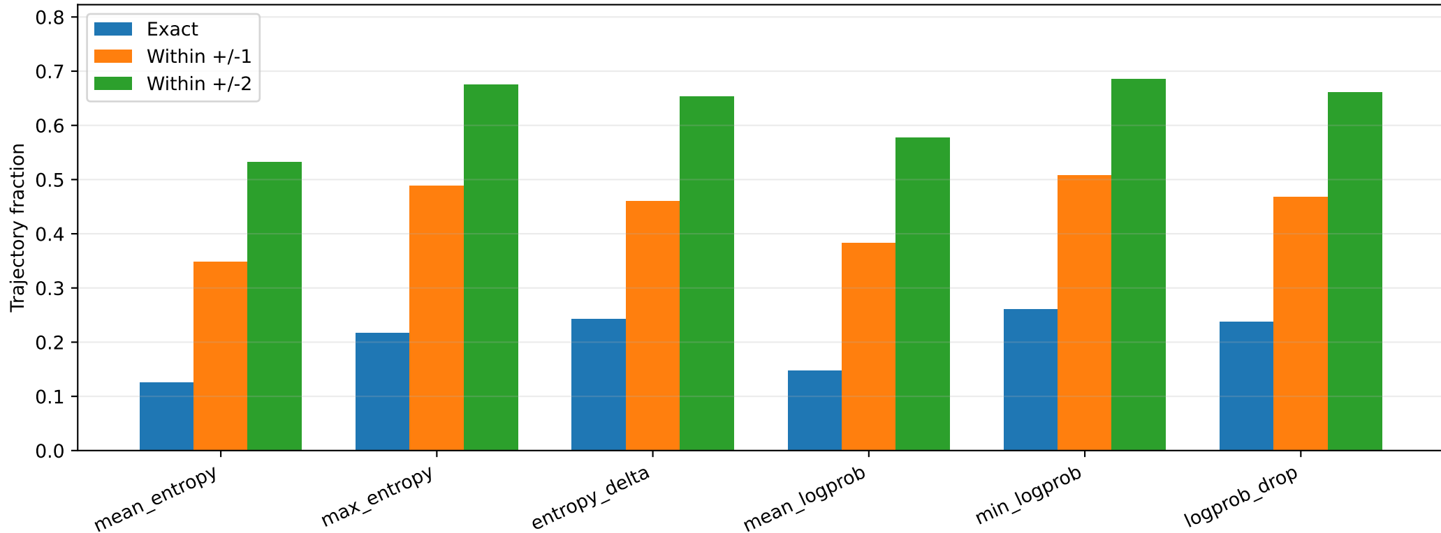
GSM8K first-error localization
