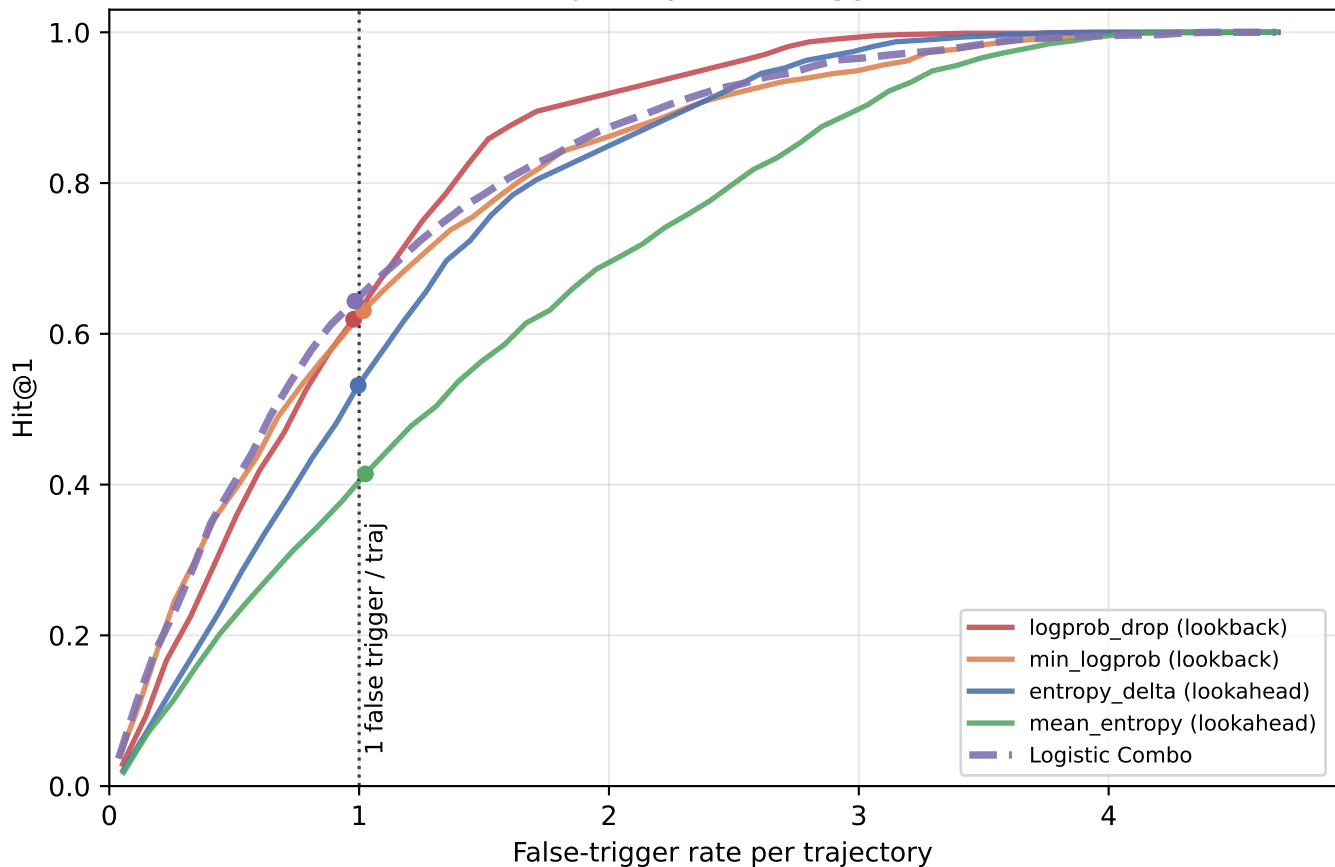
GSM8K Trajectory-Level Trigger Hit-Rate
