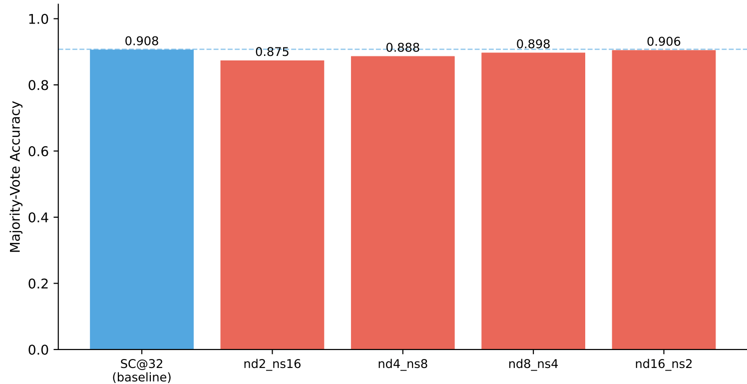
Accuracy: SC@32 vs Rollback Configs (B=32)
