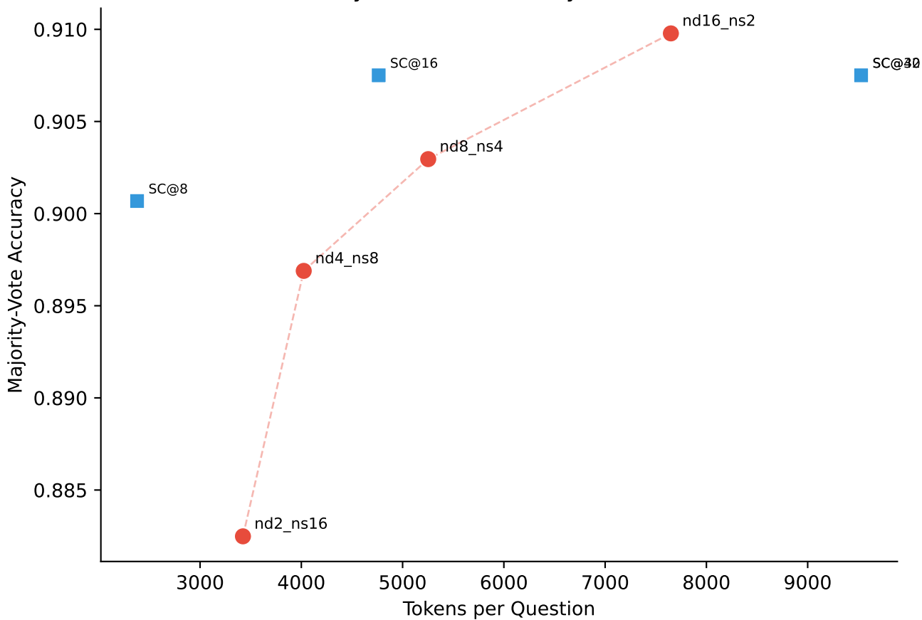
Efficiency Frontier: Accuracy vs Token Cost
