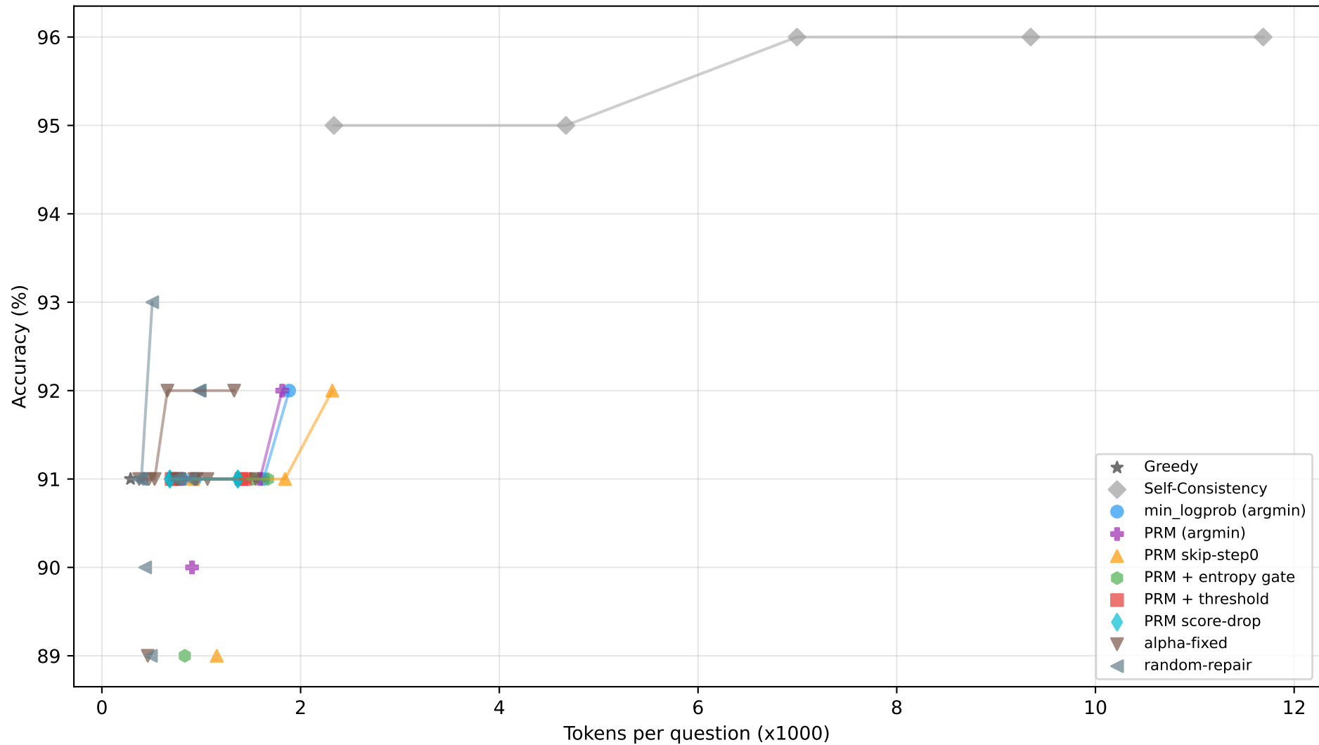
Qwen2.5-3B-Instruct on GSM8K: Acc vs Compute
