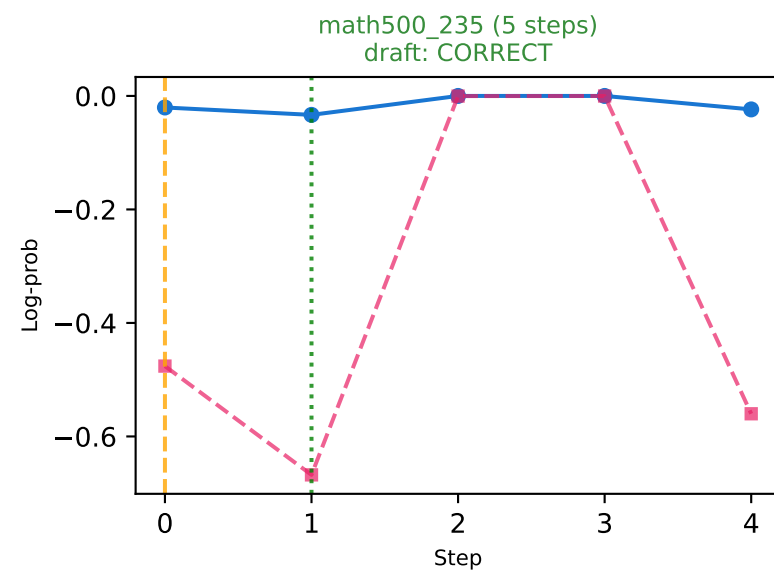
Logprob Step Curves (MATH-500, Qwen2.5-3B) | orange=PRM rollback, green=logprob argmin
