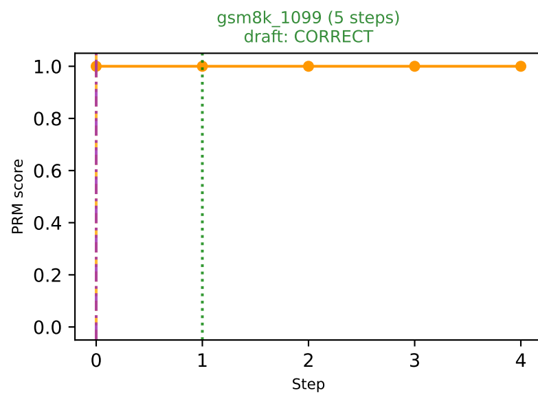
PRM Score Step Curves (GSM8K, Qwen2.5-3B) | orange=PRM, green=min_lp, purple=mean_NLL
