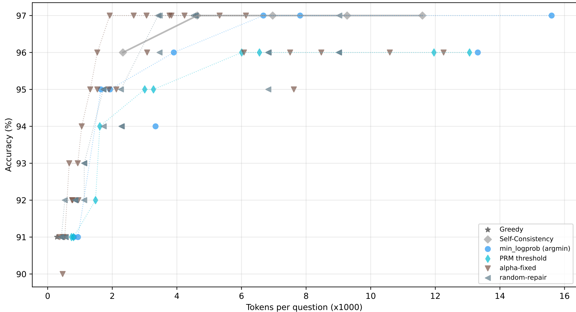
Qwen2.5-3B-Instruct on GSM8K: Acc vs Compute [PRM scoring tokens INCLUDED]
