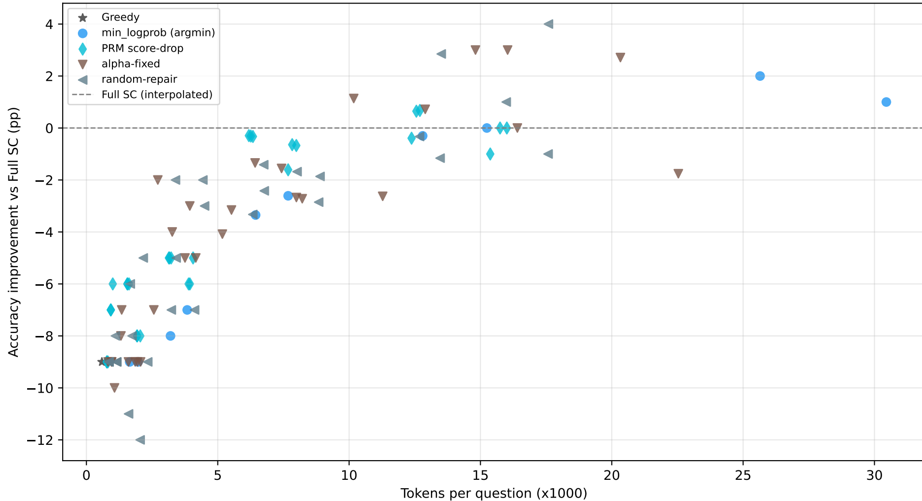
Acc improvement over Full SC at same token budget [PRM scoring tokens EXCLUDED]
