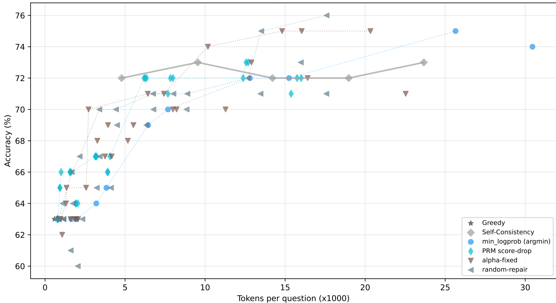
Qwen2.5-3B-Instruct on GSM8K: Acc vs Compute [PRM scoring tokens EXCLUDED]
