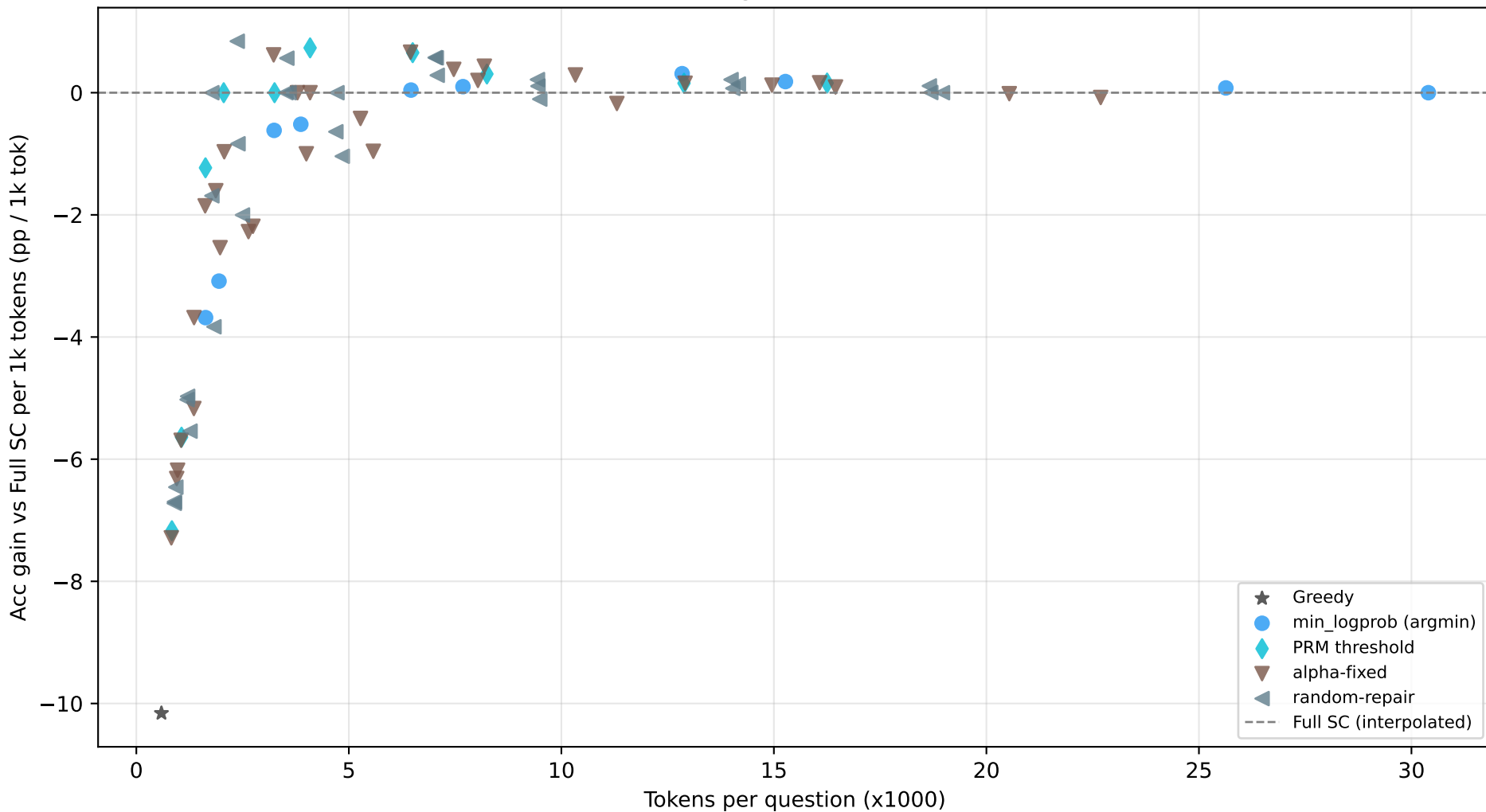
Efficiency: acc gain over Full SC per 1k tokens [PRM scoring tokens EXCLUDED]
