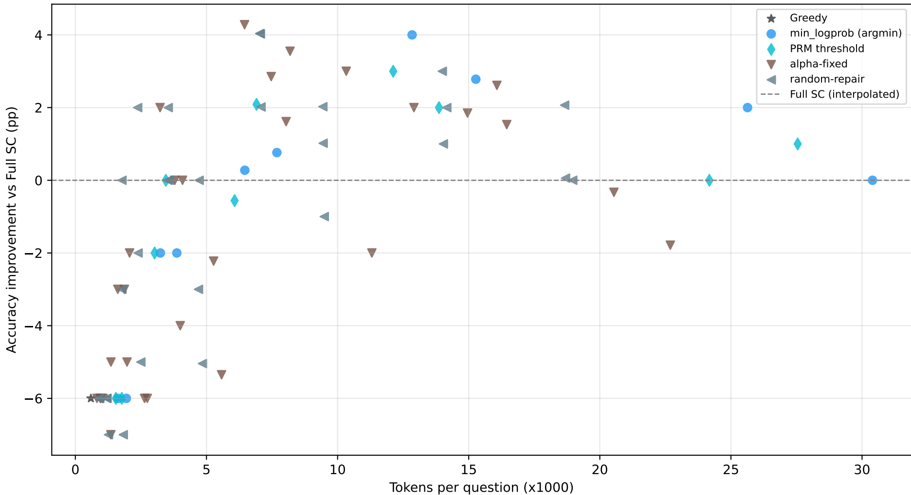
Acc improvement over Full SC at same token budget [PRM scoring tokens INCLUDED]
