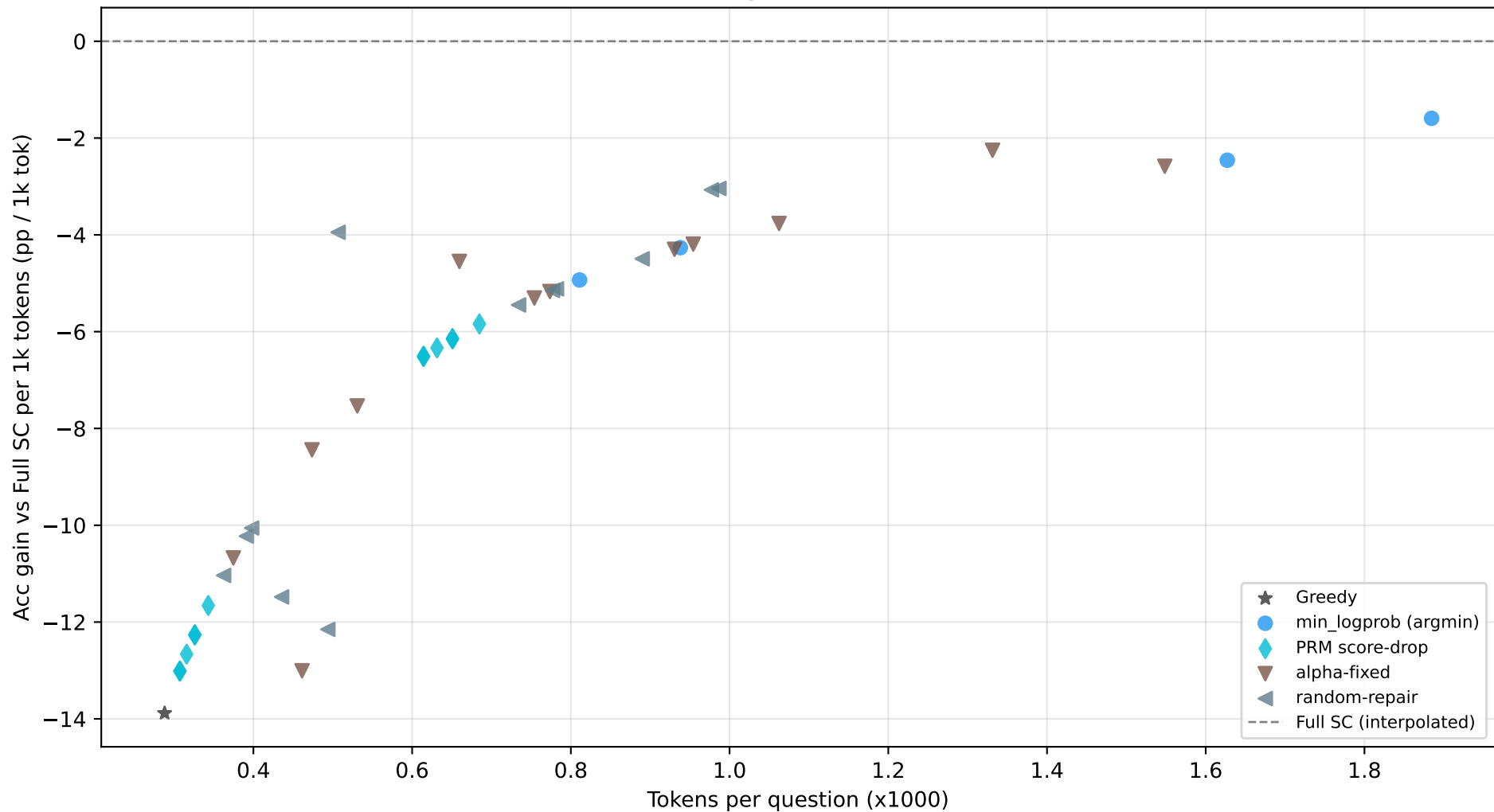
Efficiency: acc gain over Full SC per 1k tokens [PRM scoring tokens INCLUDED]
