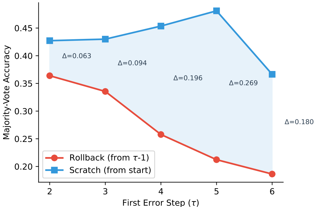
Accuracy by Error Position
