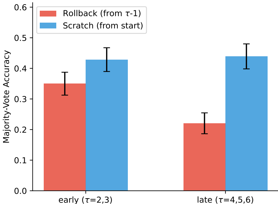
Rollback Resample vs From-Scratch Resample
