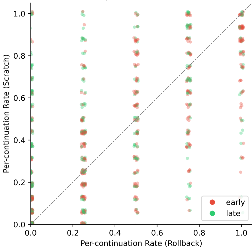
Per-sample: Rollback vs Scratch
