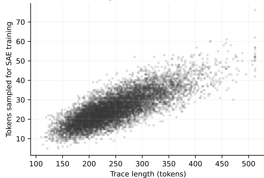
Full sequence token-uniform Spearman r = 0.768
