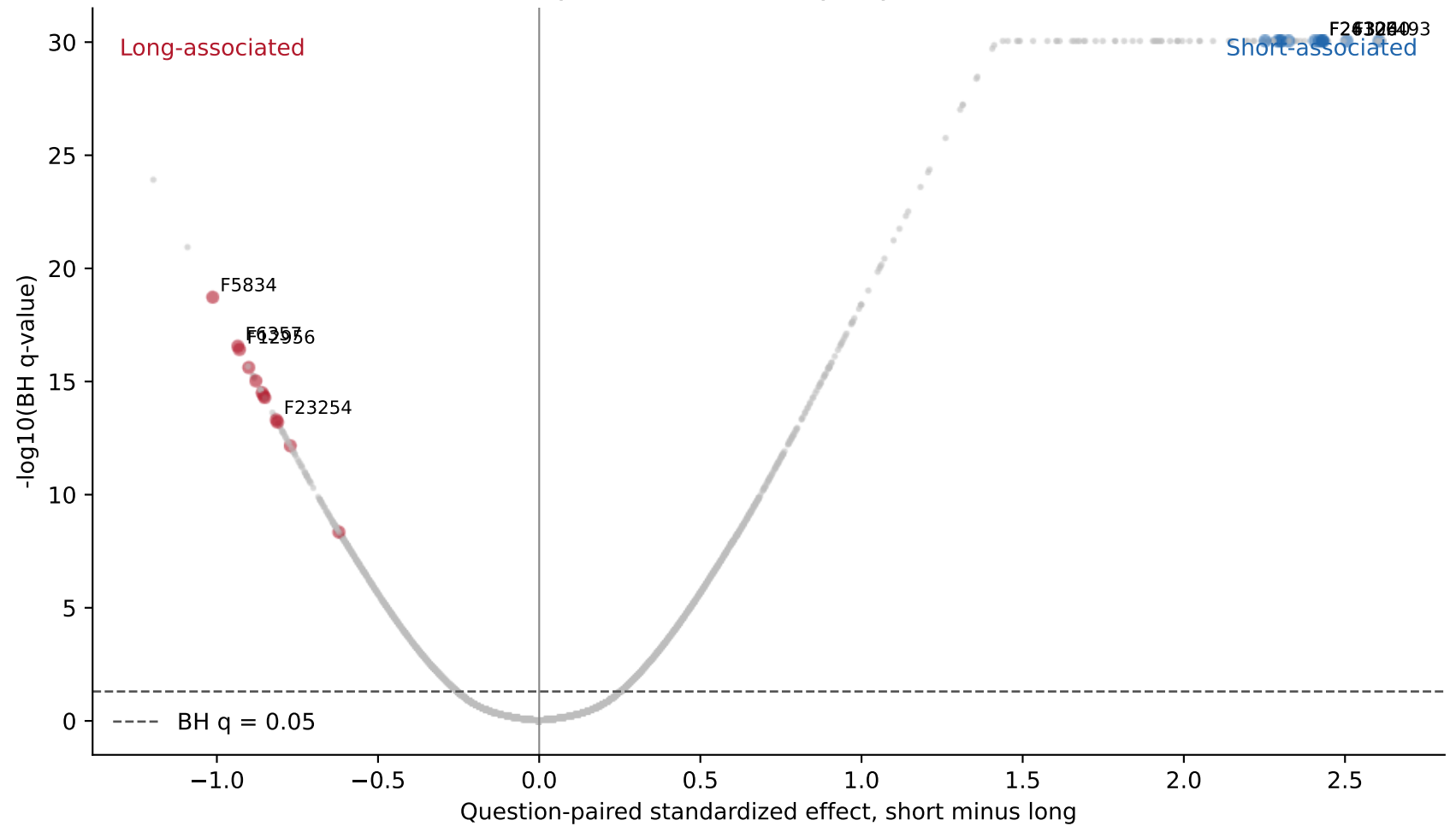
Primary SAE dev discovery (layer 17, k=64)
