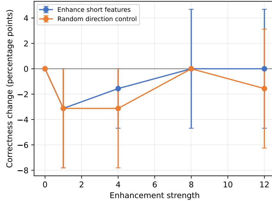
Stronger SAE intervention: paired teacher dose response 64 traces per condition; pointwise 95% question-bootstrap intervals; exploratory
