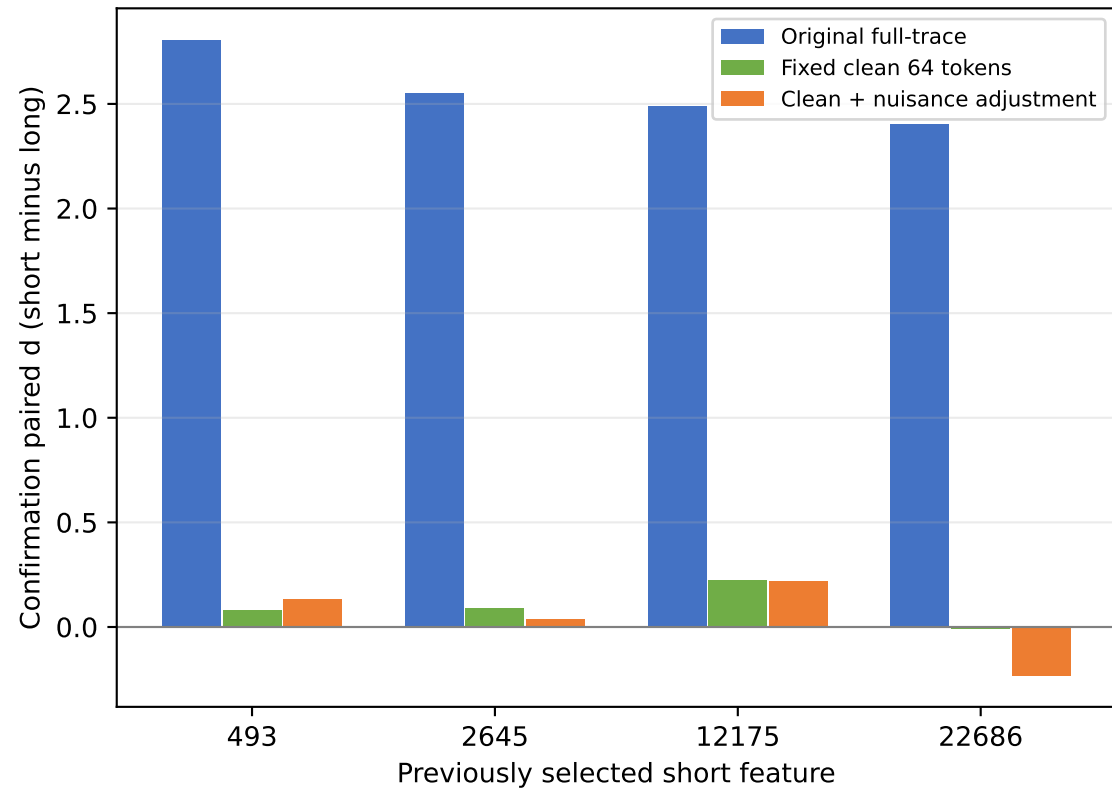
SAE length association after removing answer / position / denominator confounds
