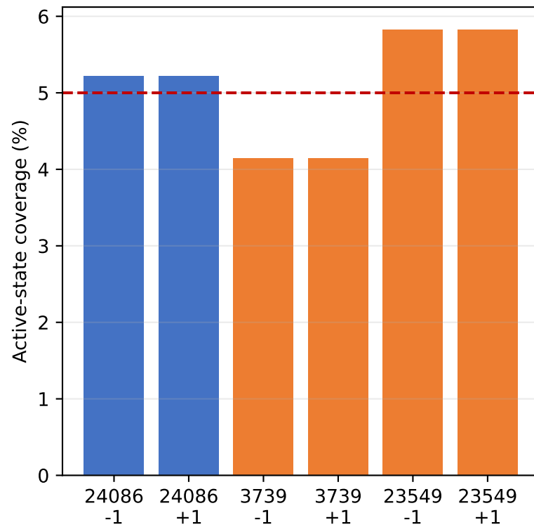
Target engagement v2: primary feature and matched random controls
