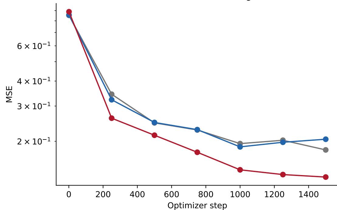
Reconstruction loss on training batches
