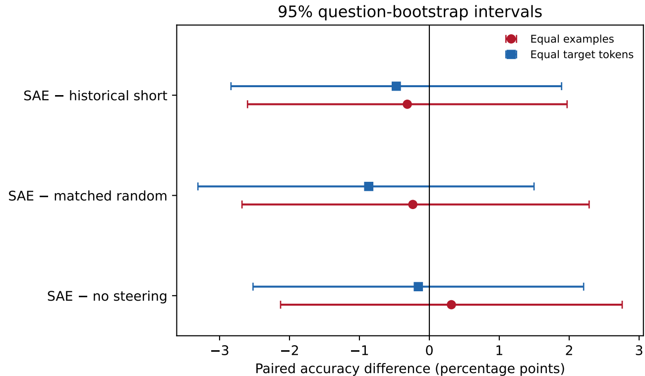
Eight student runs: same question support, seed 17, full 1,269-question evaluation
