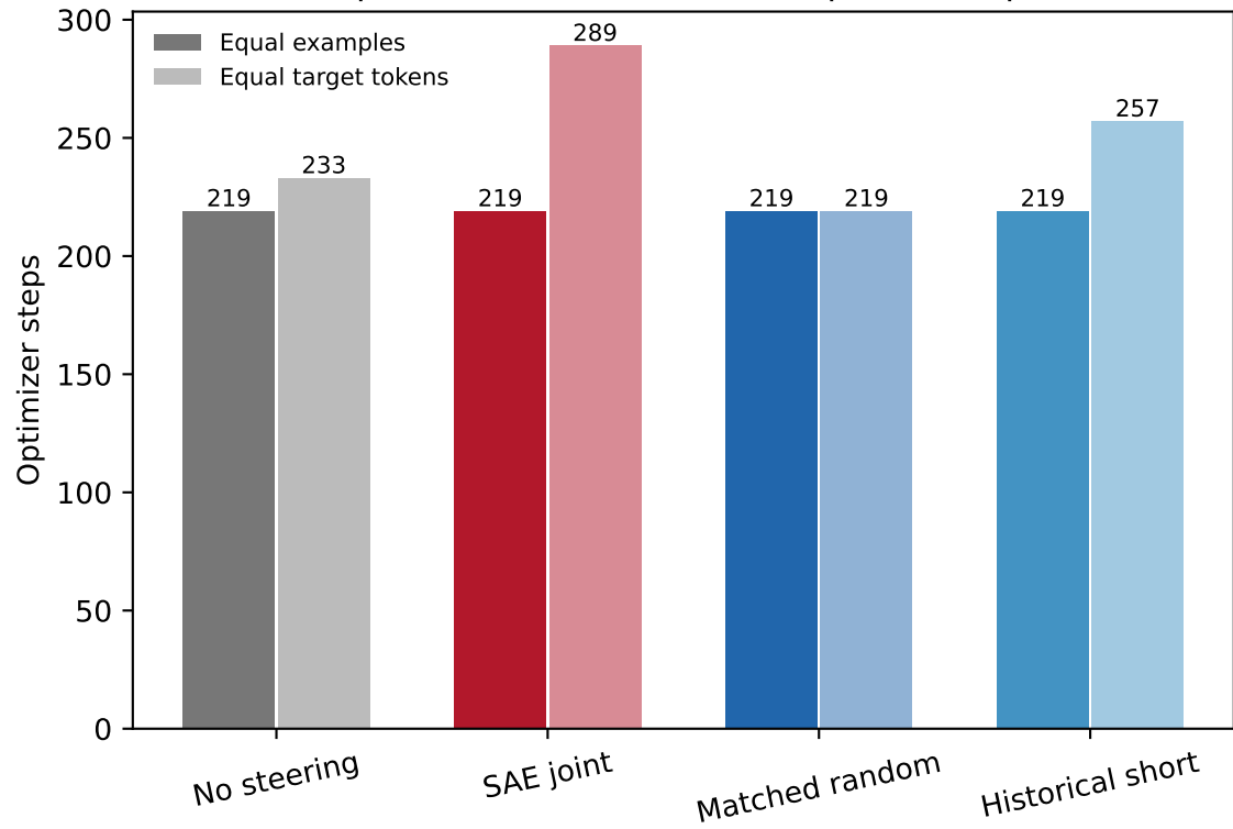
Equal token counts do not equalize steps
