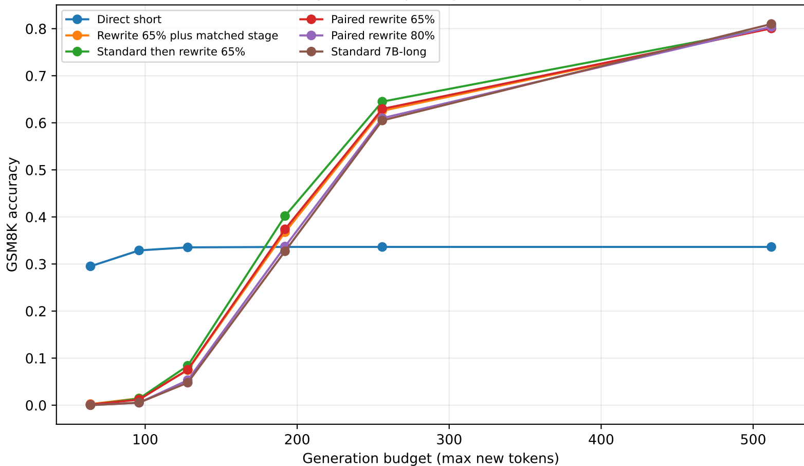
Accuracy under explicit generation budgets
