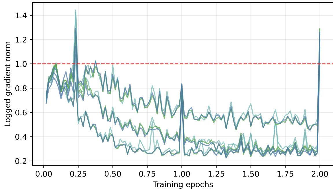
Gradient stability
