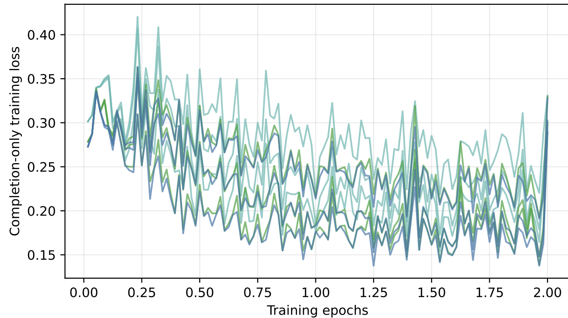
Loss trajectory
