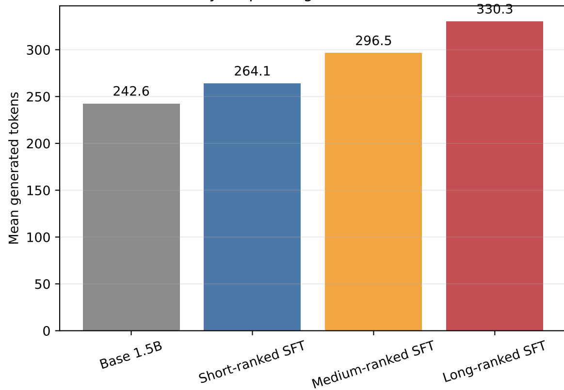
Greedy output length, max 512 tokens
