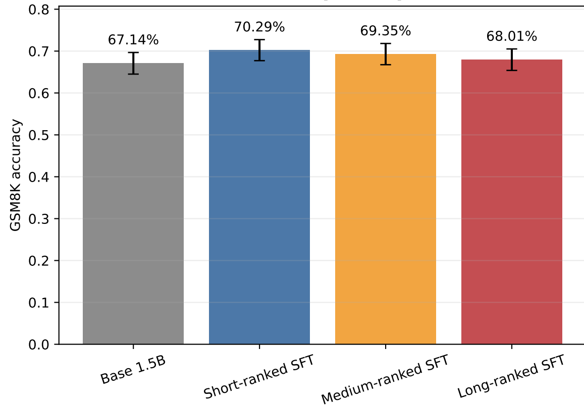
Locked GSM8K test[50:1319], n=1269
