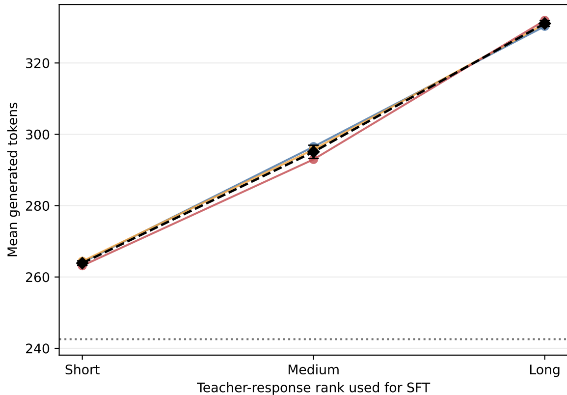
Student response length across training seeds
