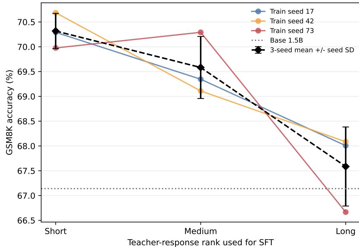
Accuracy across training seeds
