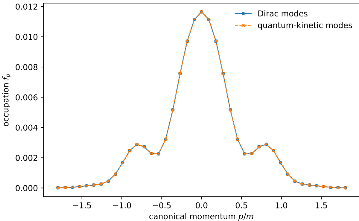
Spectrum from two separated Sauter pulses
