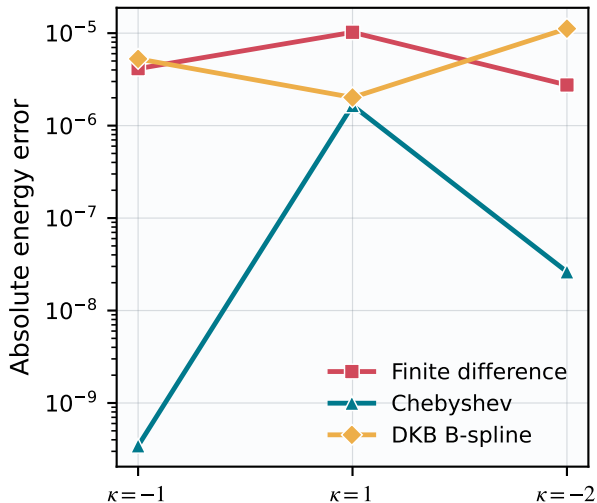
(b) Absolute error relative to shooting
