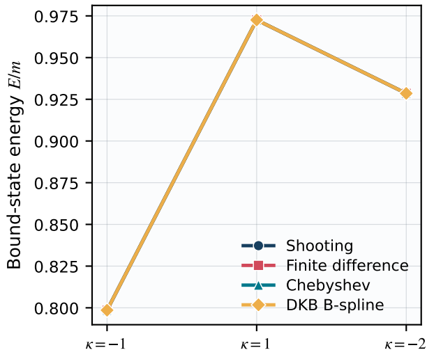
(a) Identified bound-state energies
