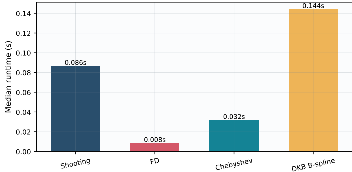
Reference runtime: one targeted P1, \kappa = -1 solve
