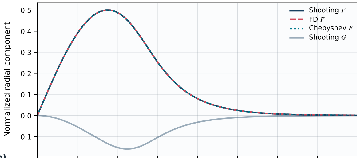
Phase-aligned spinors for P1, \kappa=-1
