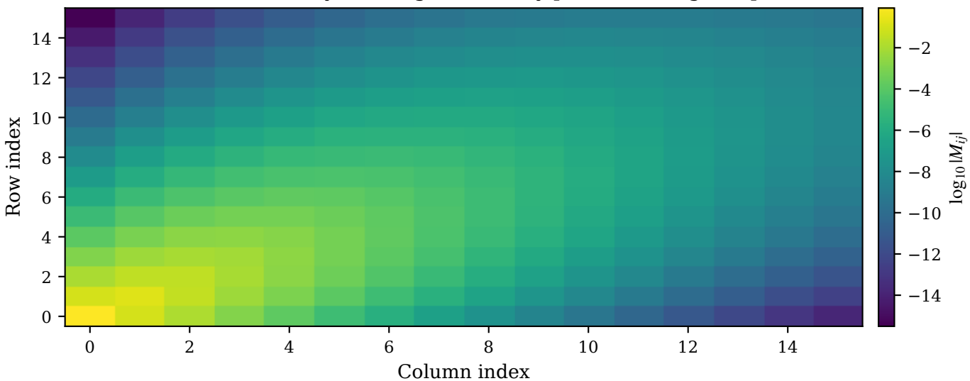
(b) Dense monodromy matrix generated by positive bidiagonal pulses
