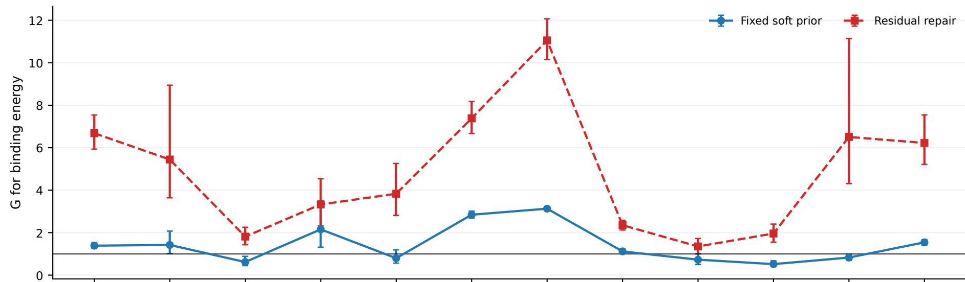
MLP ensemble
