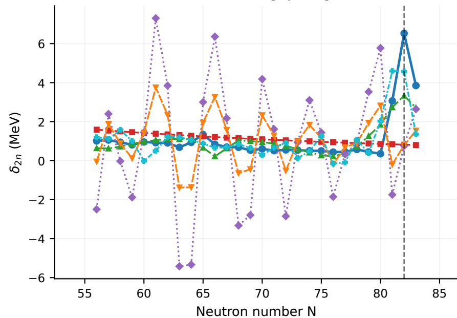
Two-neutron shell-gap diagnostic
