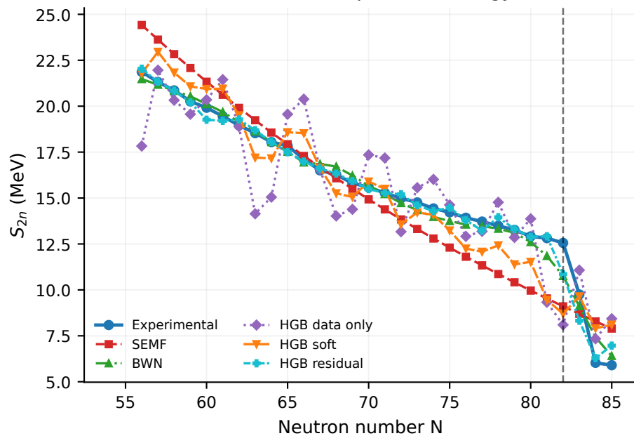
Two-neutron separation energy
