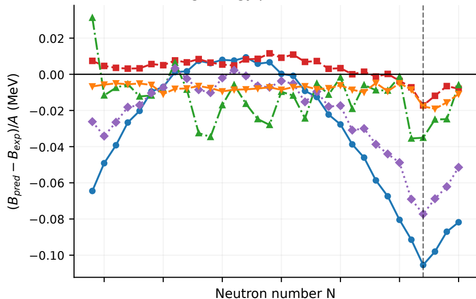
Two-neutron shell-gap diagnostic
