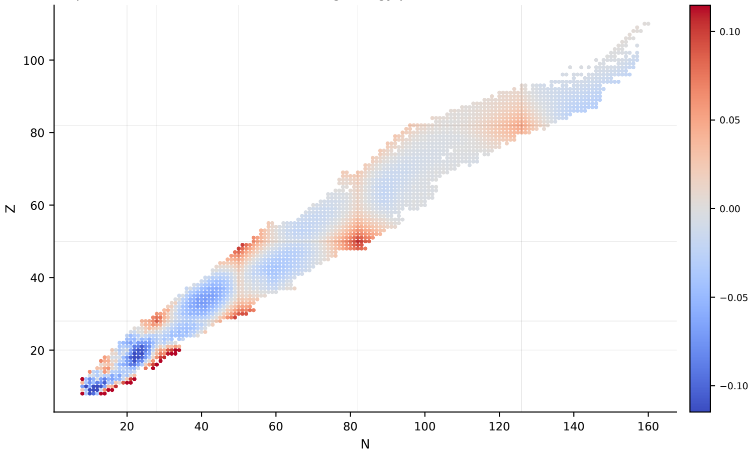
Experimental minus fitted SEMF binding energy per nucleon (99% scale \pm 0.115 MeV)
