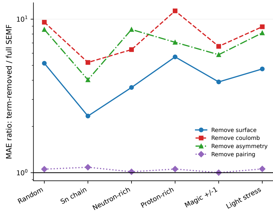
One-term-removal diagnostics
