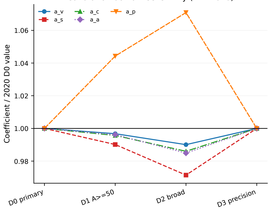
Calibration-domain sensitivity (AME2020)
